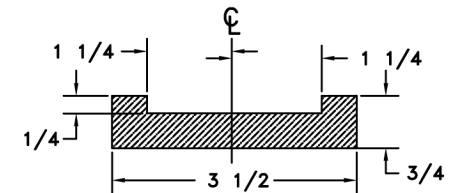
TOP: CROSS SECTION SCALE: FULL
