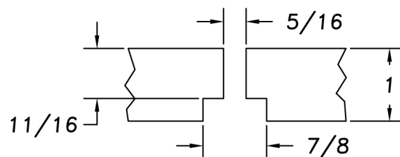
COUNTERBORE DETAIL
