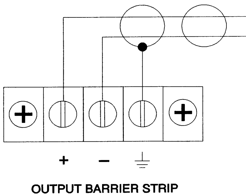
Figure 2 Output Connections
