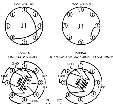
Figure 3. Socket Wiring for Transformer-Isolated Input Using 15095A Line Transformer
