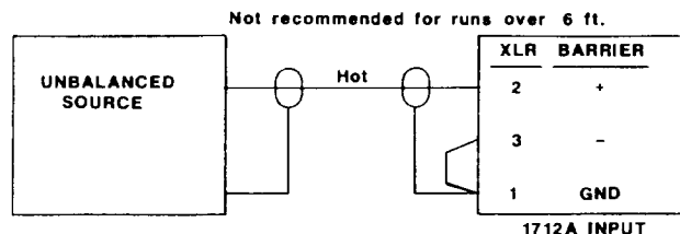
Figure 2. Typical Input Connections
