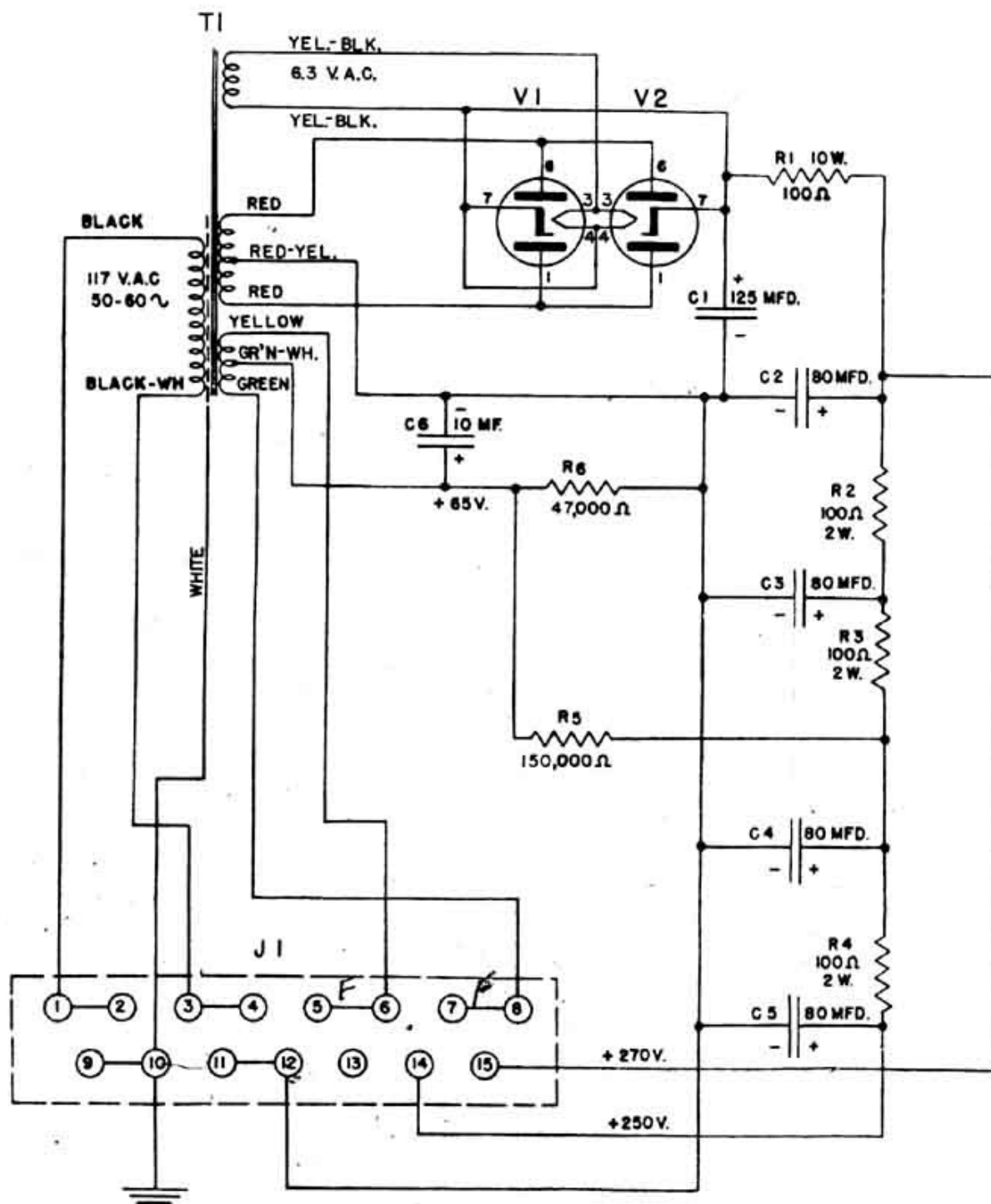
ALTEC LANSING P522B POWER SUPPLY
