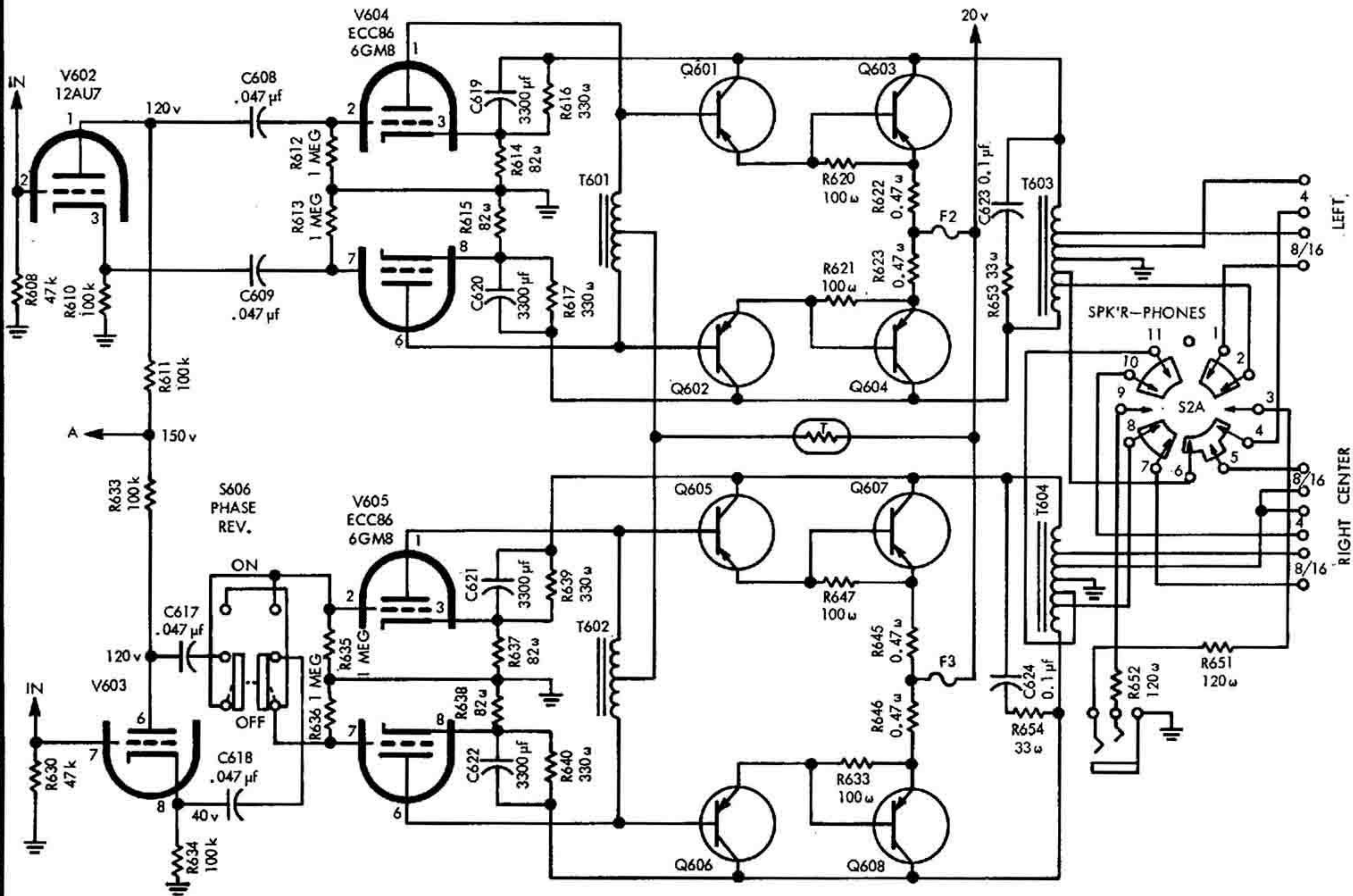
Schematic of the output and driving stages of the "Astro."
