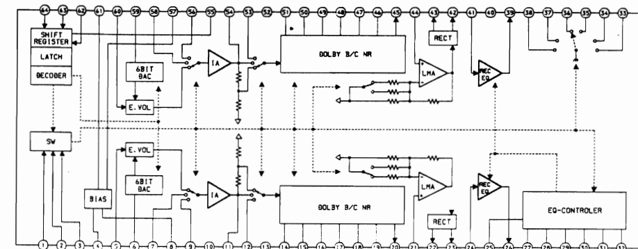
IC, HA12155NT - 01
