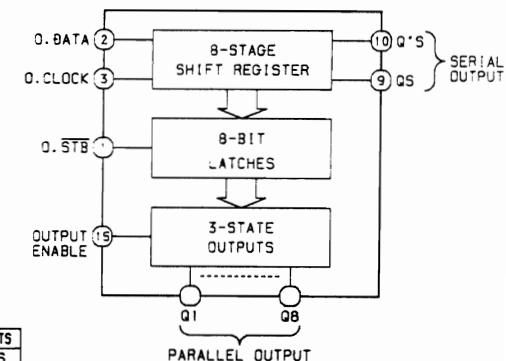
IC, BU4094B
