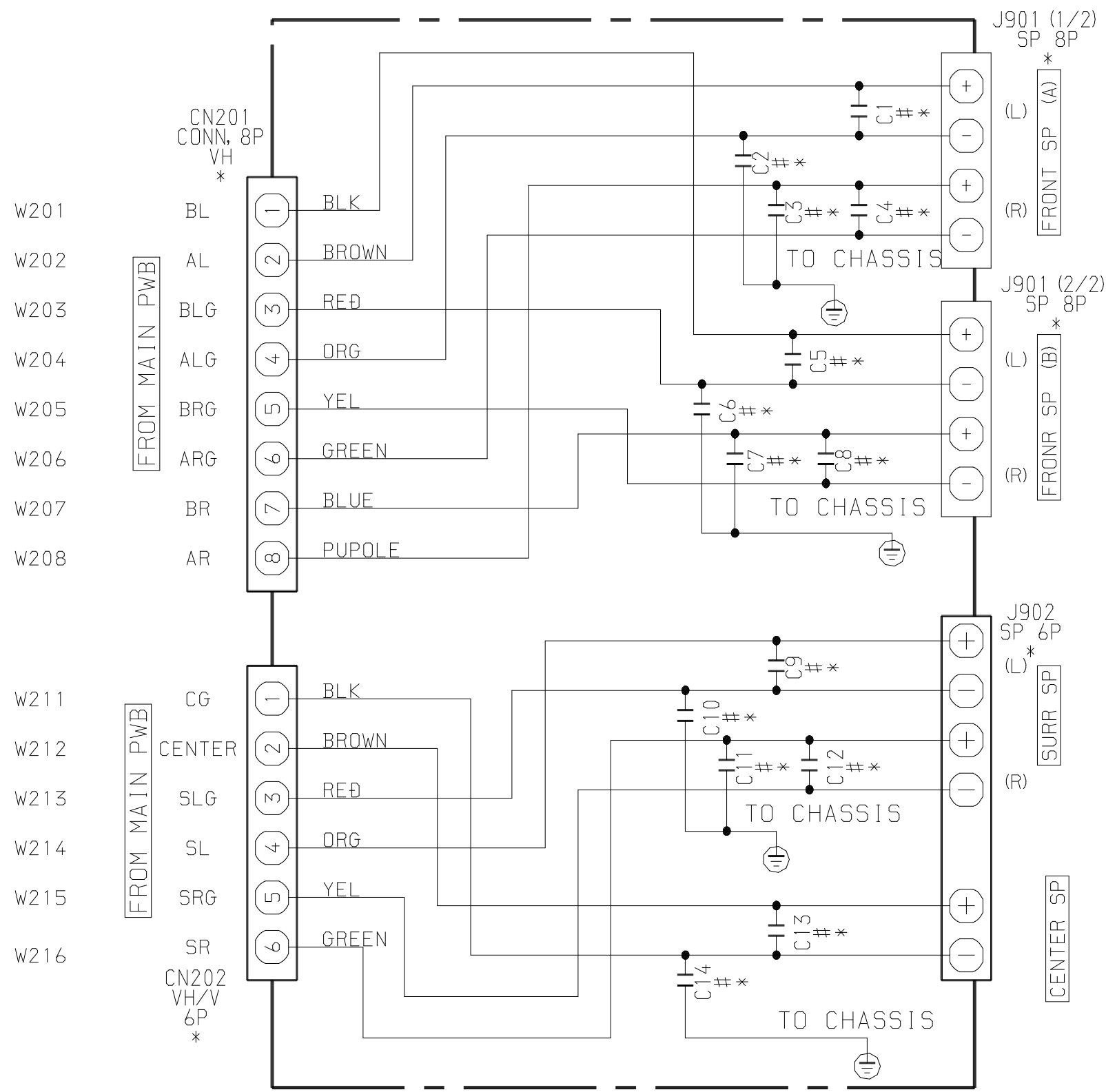
SCHEMATIC DIAGRAM – 7 (SPEAKER)
