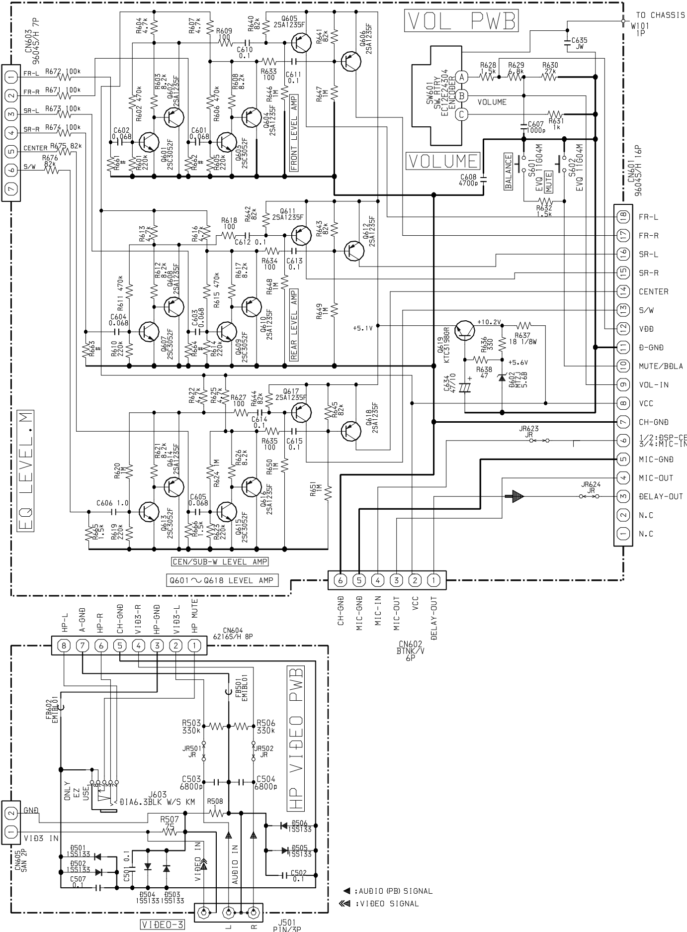
SCHEMATIC DIAGRAM – 5 (HP VIDEO / GEQ / VOL)
