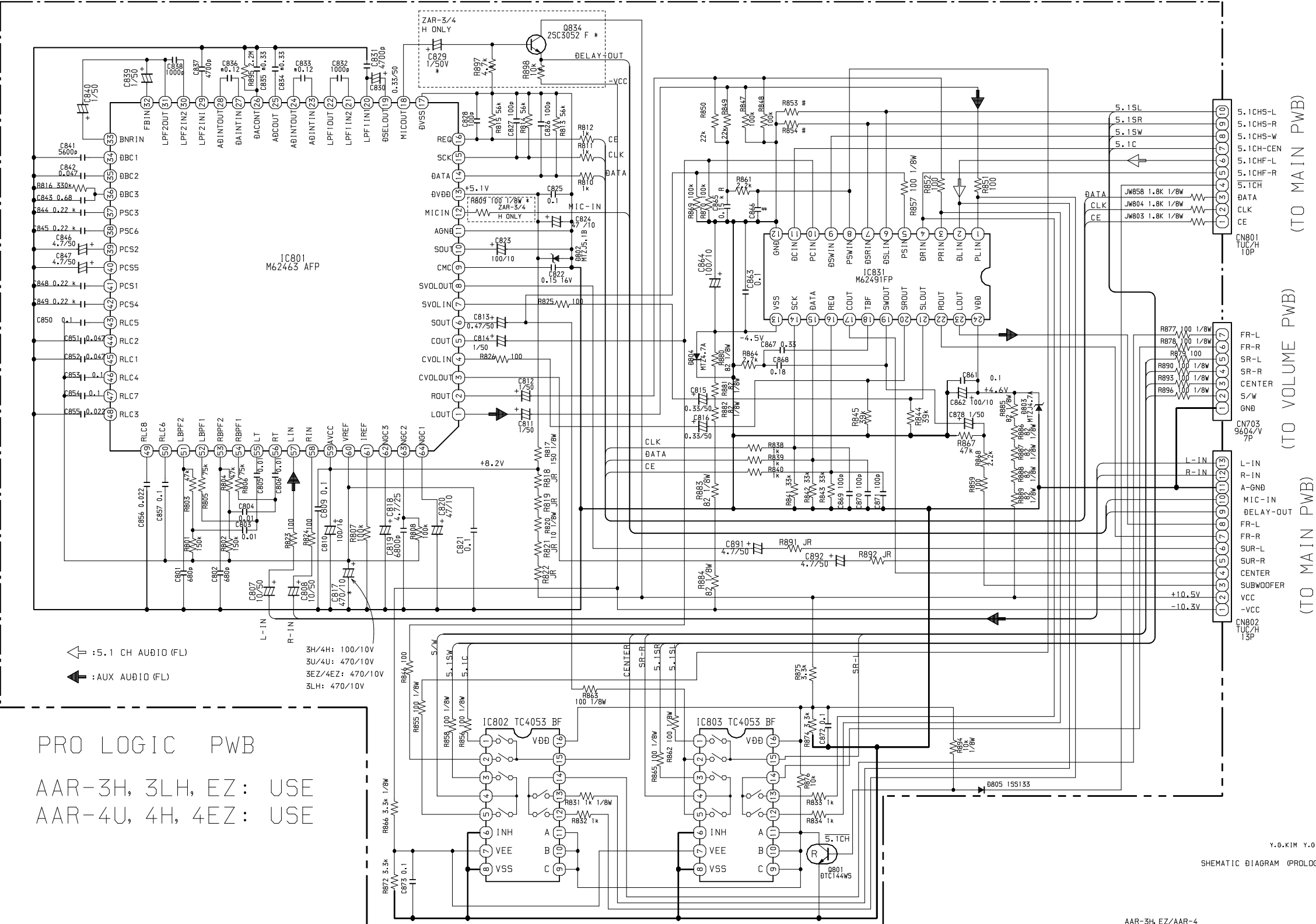
SCHEMATIC DIAGRAM – 6 (PROLOGIC)
