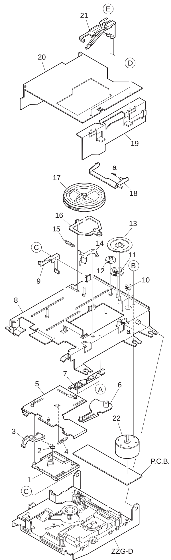
MECHANISM EXPLODED VIEW 1/1 (7ZG8)
