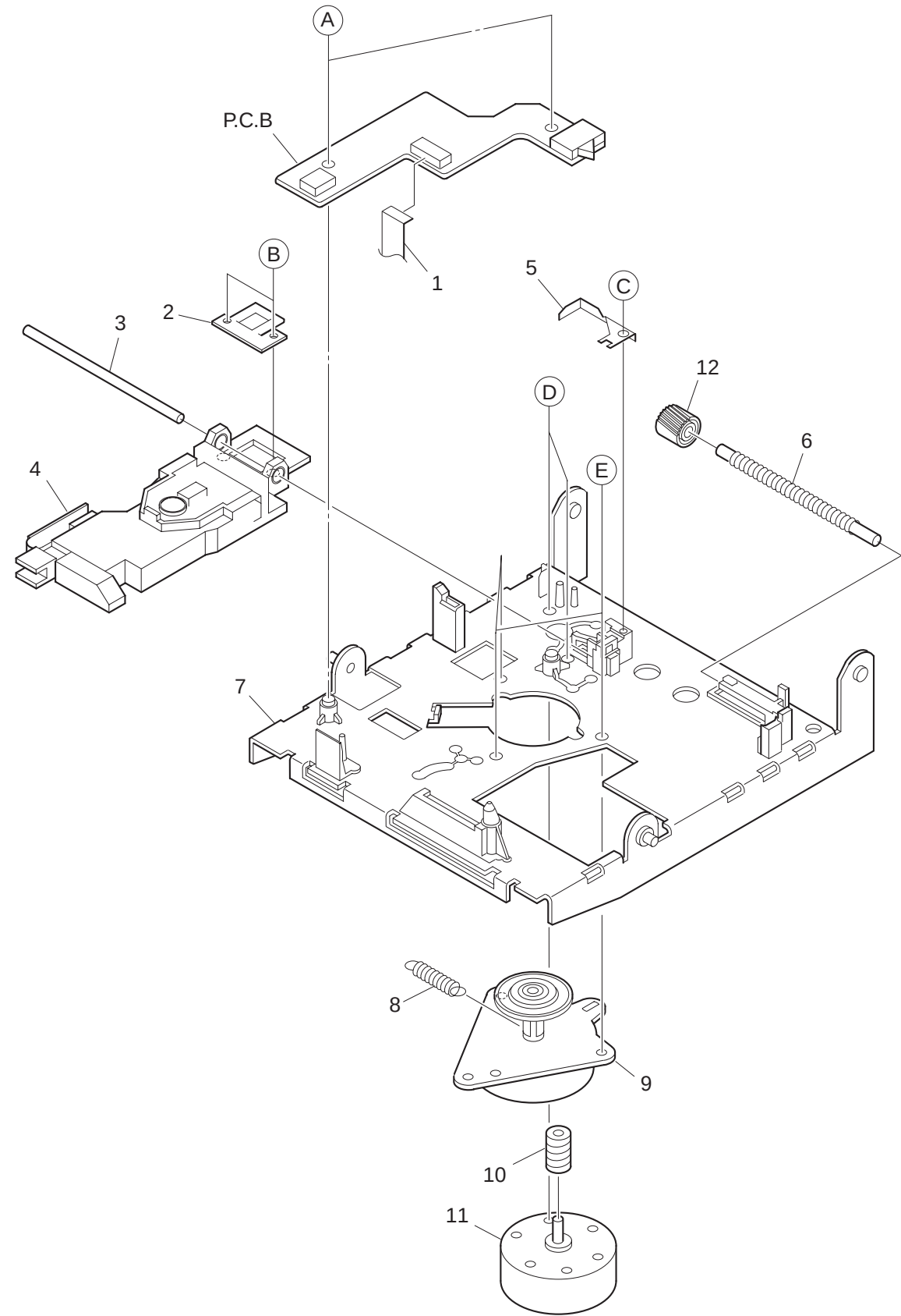
MECHANISM EXPLODED VIEW 1/1 (ZZG-D)
