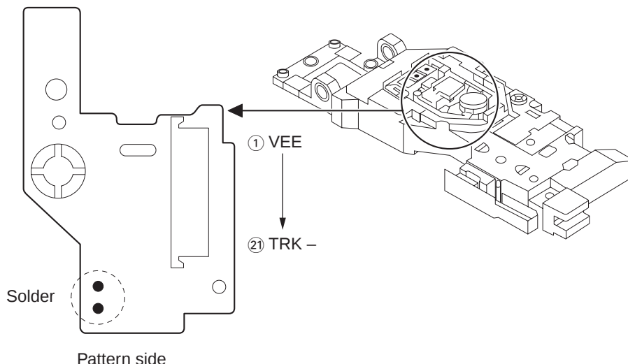
MD PICKUP Assy P.C.B.
