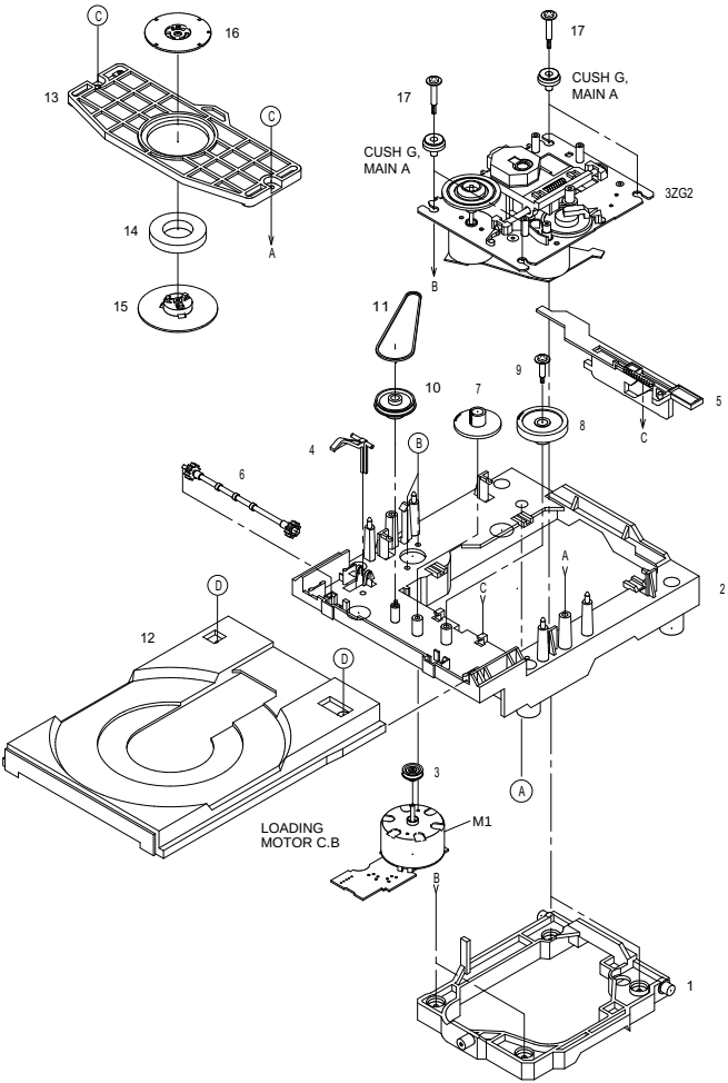
CD MECHANISM EXPLODED VIEW 1/2
