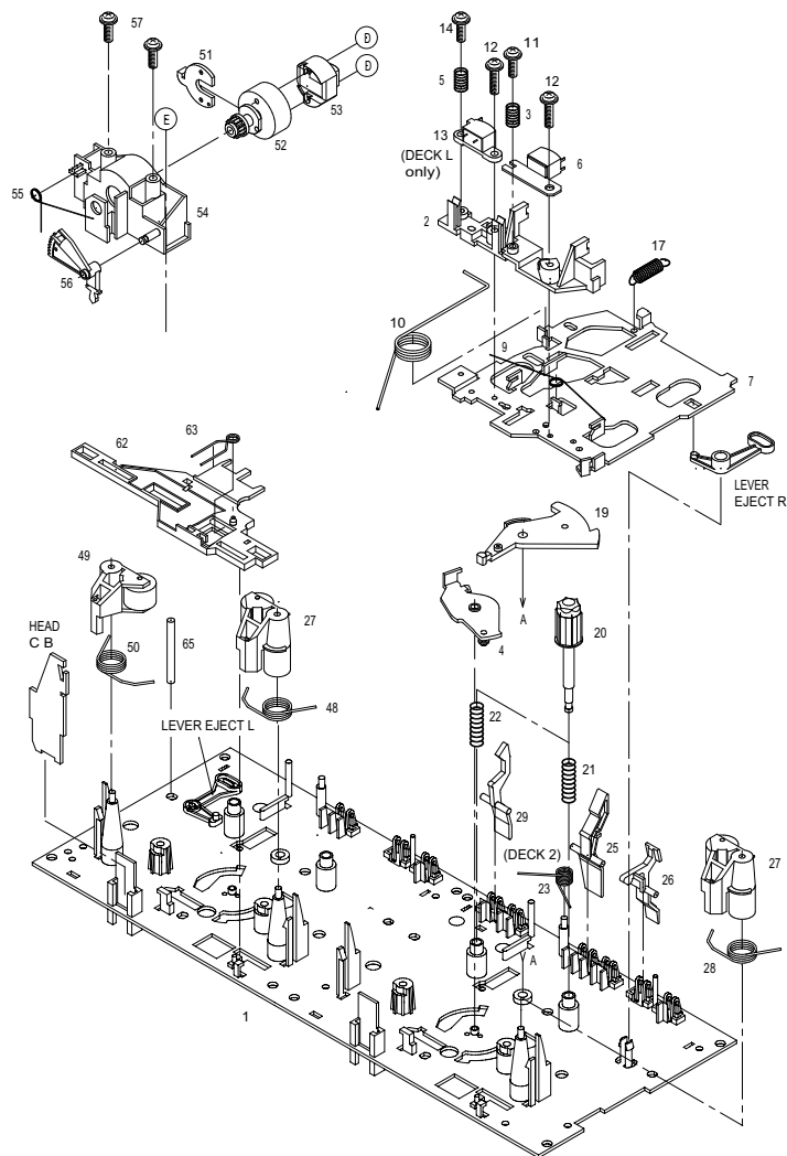
TAPE MECHANISM EXPLODED VIEW 1/1
