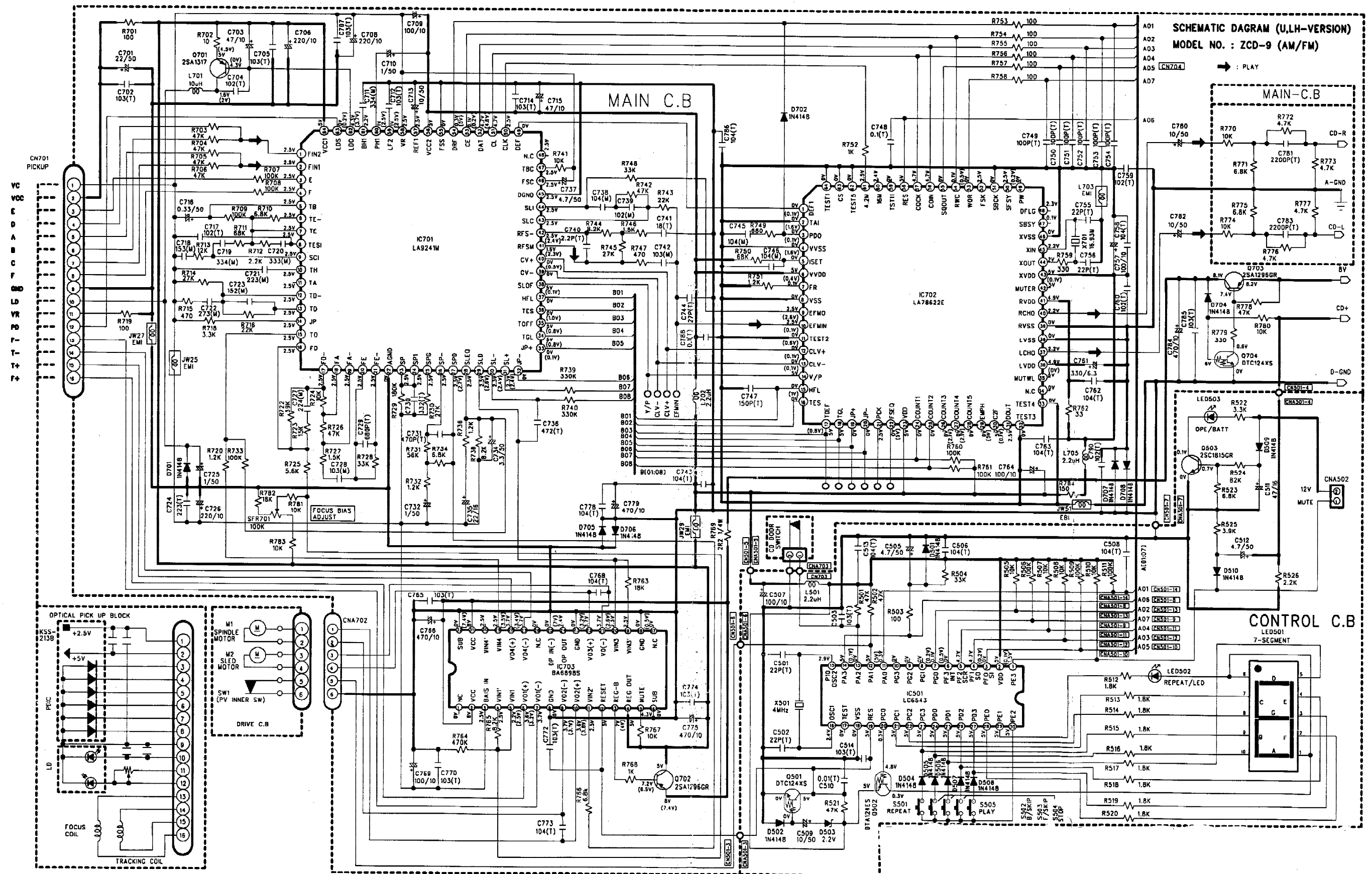
SCHEMATIC DIAGRAM - 4 (MAIN CD / CONTROL: 228LH)
