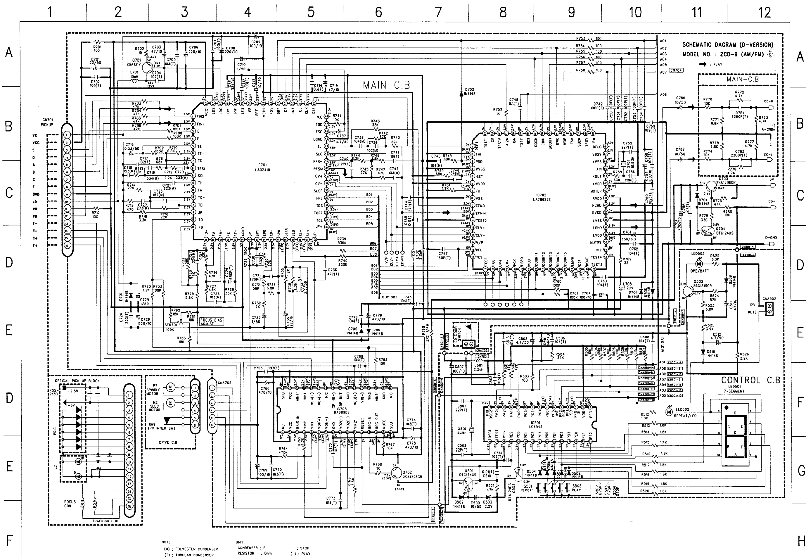
SCHEMATIC DIAGRAM - 2 (MAIN CD / CONTROL: 217D)
