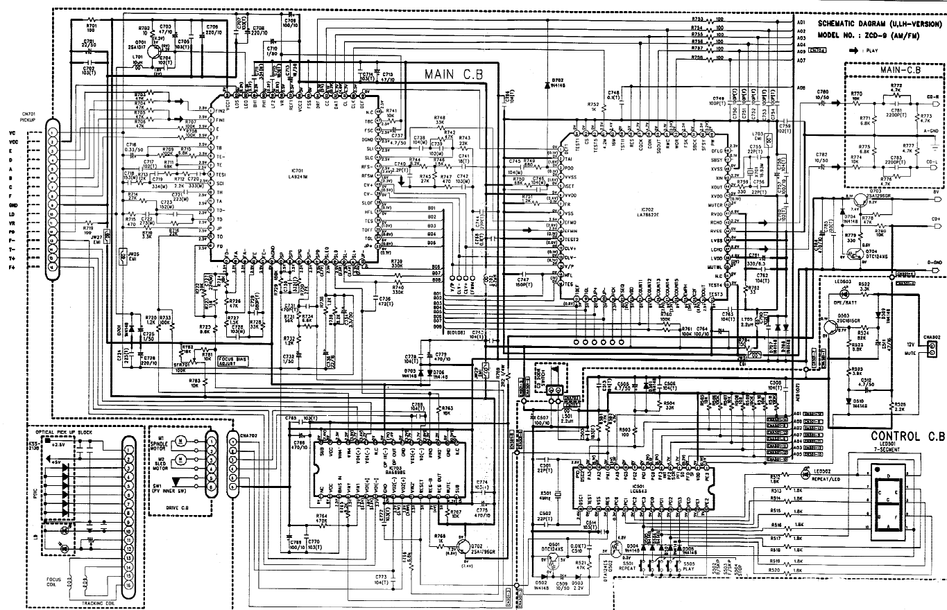
SCHEMATIC DIAGRAM – 2 (MAIN CD / CONTROL)
