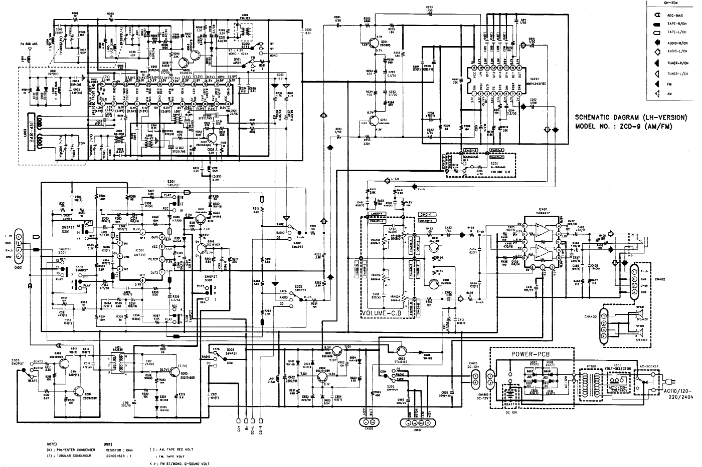
SCHEMATIC DIAGRAM - 1 (MAIN)
