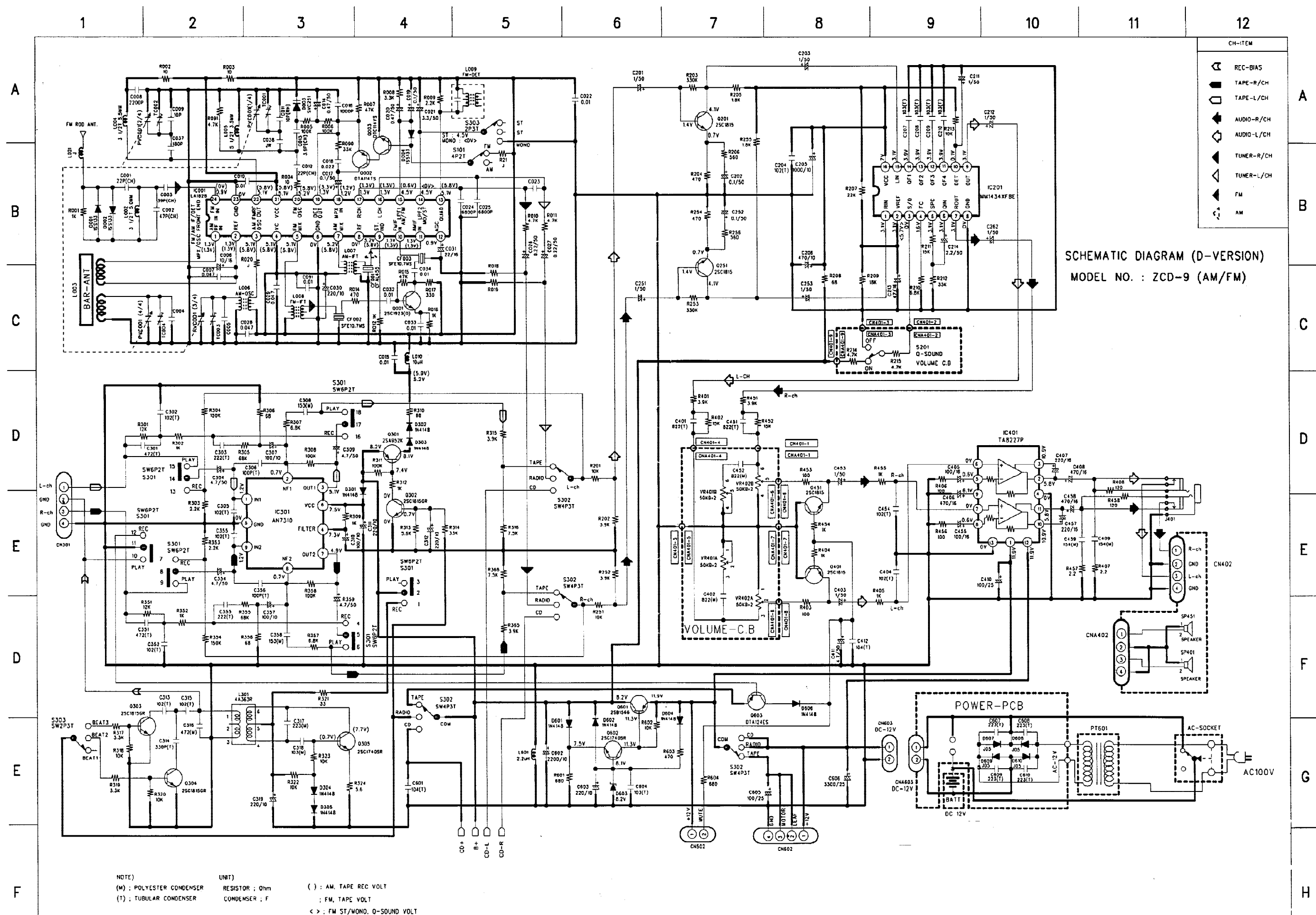
SCHEMATIC DIAGRAM - 1 (MAIN: 217D)
