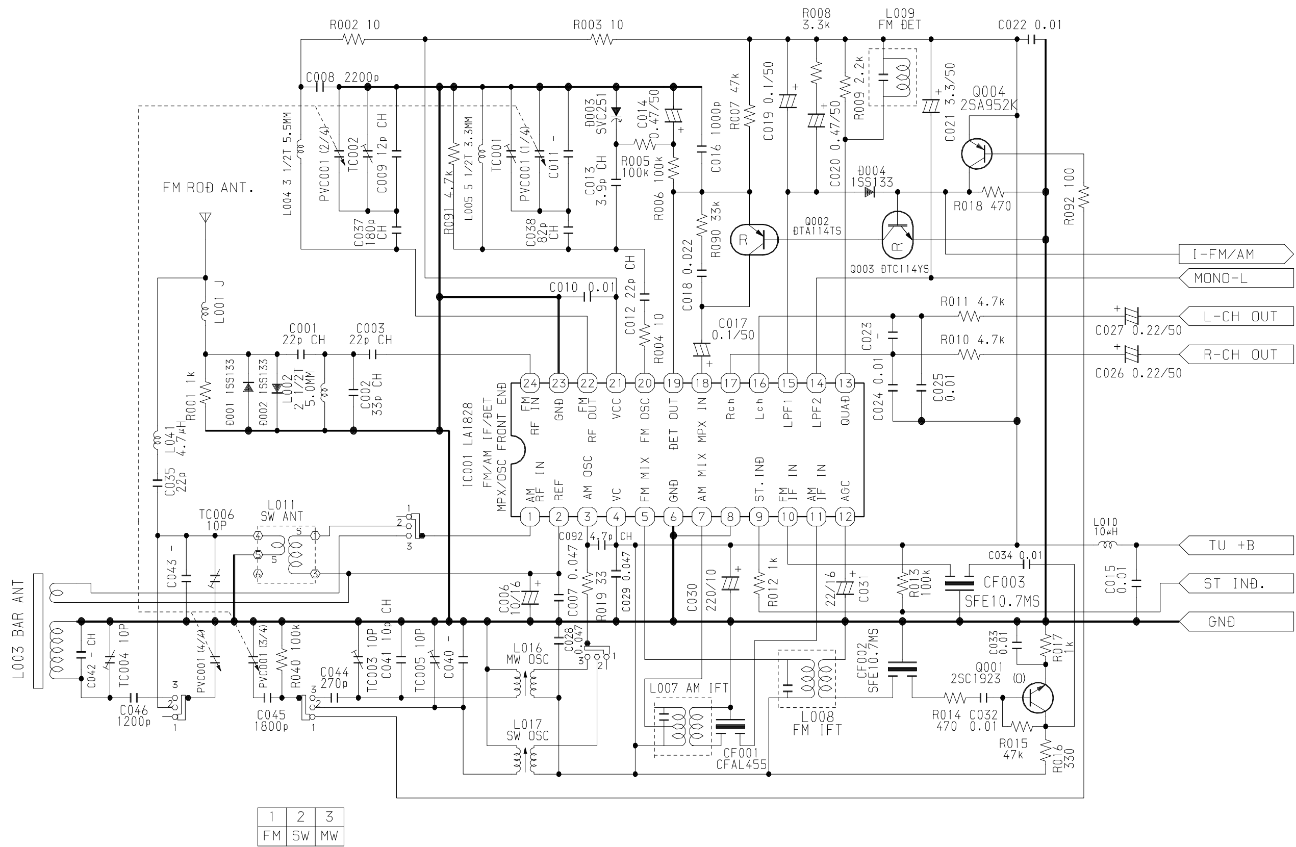
SCHEMATIC DIAGRAM – 6 (TUNER: HR)
