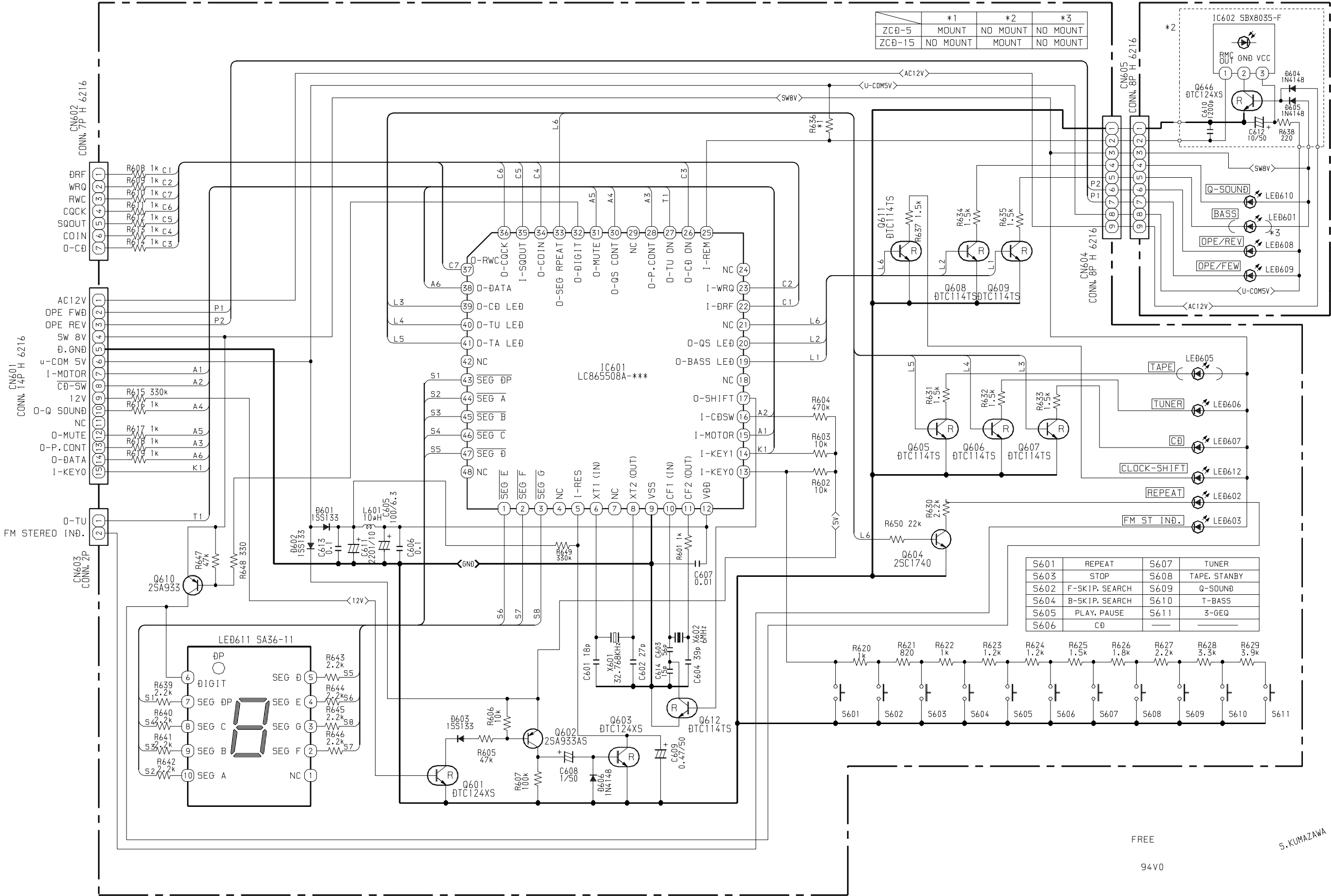
SCHEMATIC DIAGRAM – 4 (FRONT 2/2)
