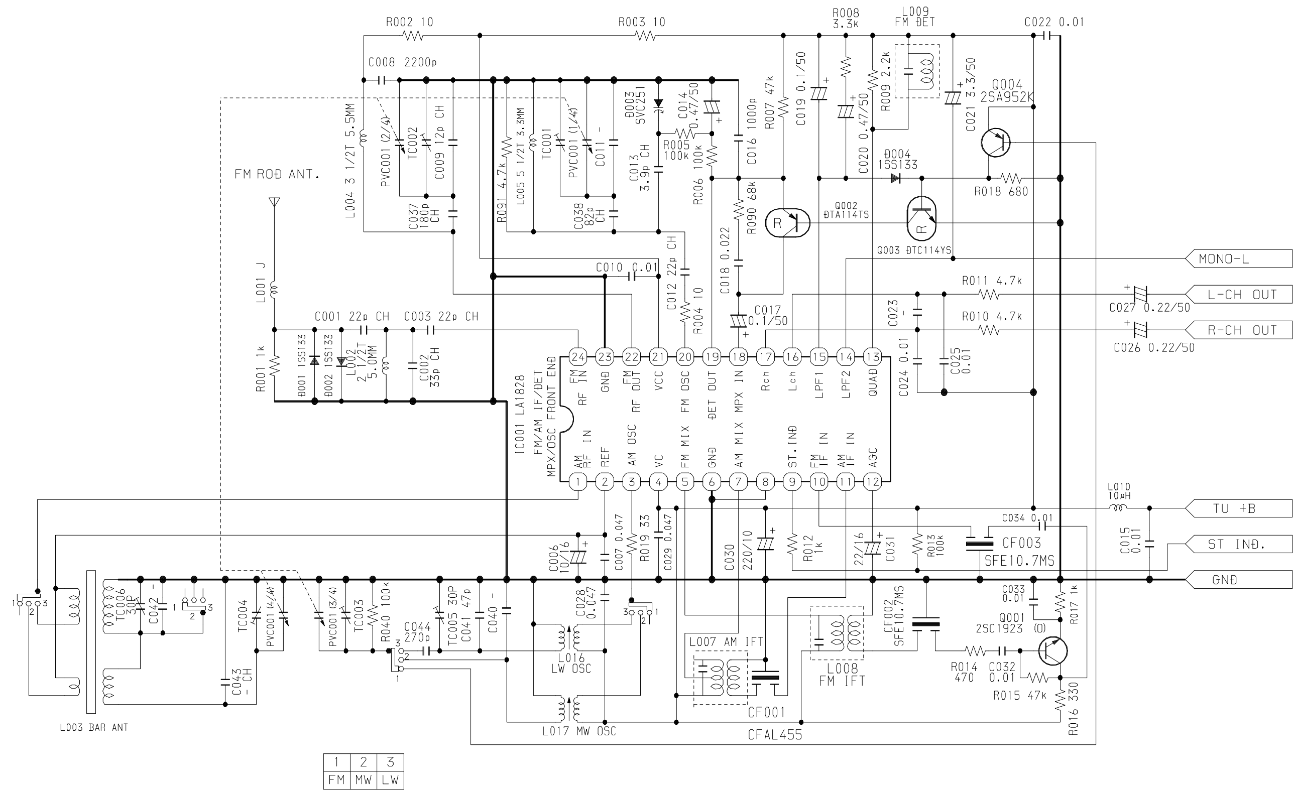
SCHEMATIC DIAGRAM – 5 (TUNER: EZ)
