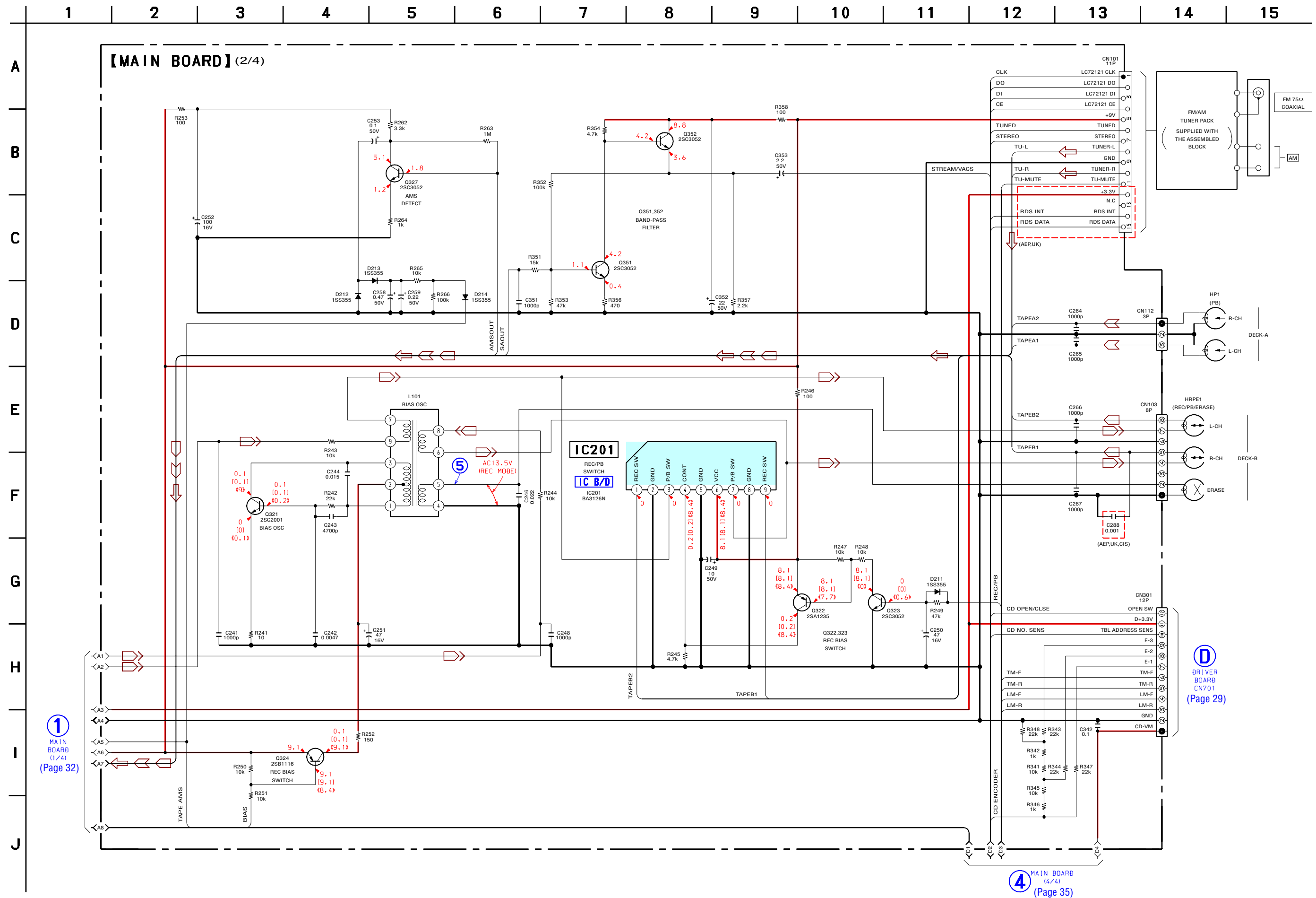
6-12. SCHEMATIC DIAGRAM – MAIN Section (2/4) – • See page 48 for IC Block Diagram. • See page 48 for Waveform.
