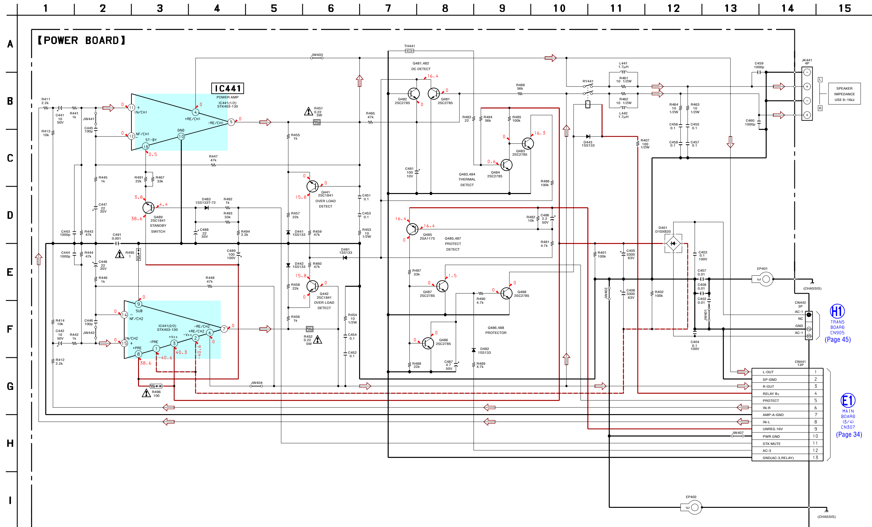
6-20. SCHEMATIC DIAGRAM – POWER AMP Section – (AEP, UK, CIS only)
