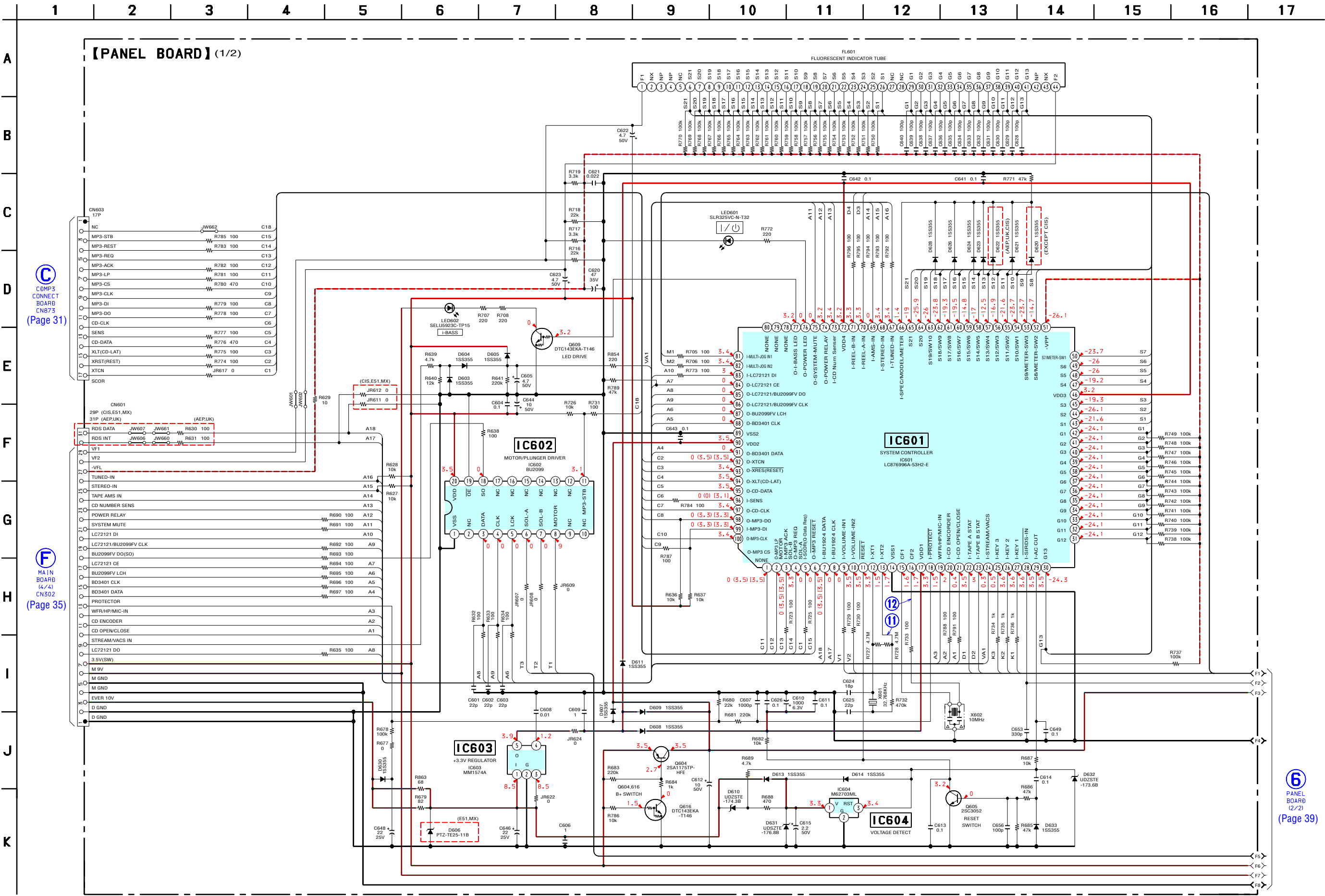
6-17. SCHEMATIC DIAGRAM – PANEL Section (1/2) – • See page 48 for Waveforms. • See page 54 for IC Pin Function Description.
