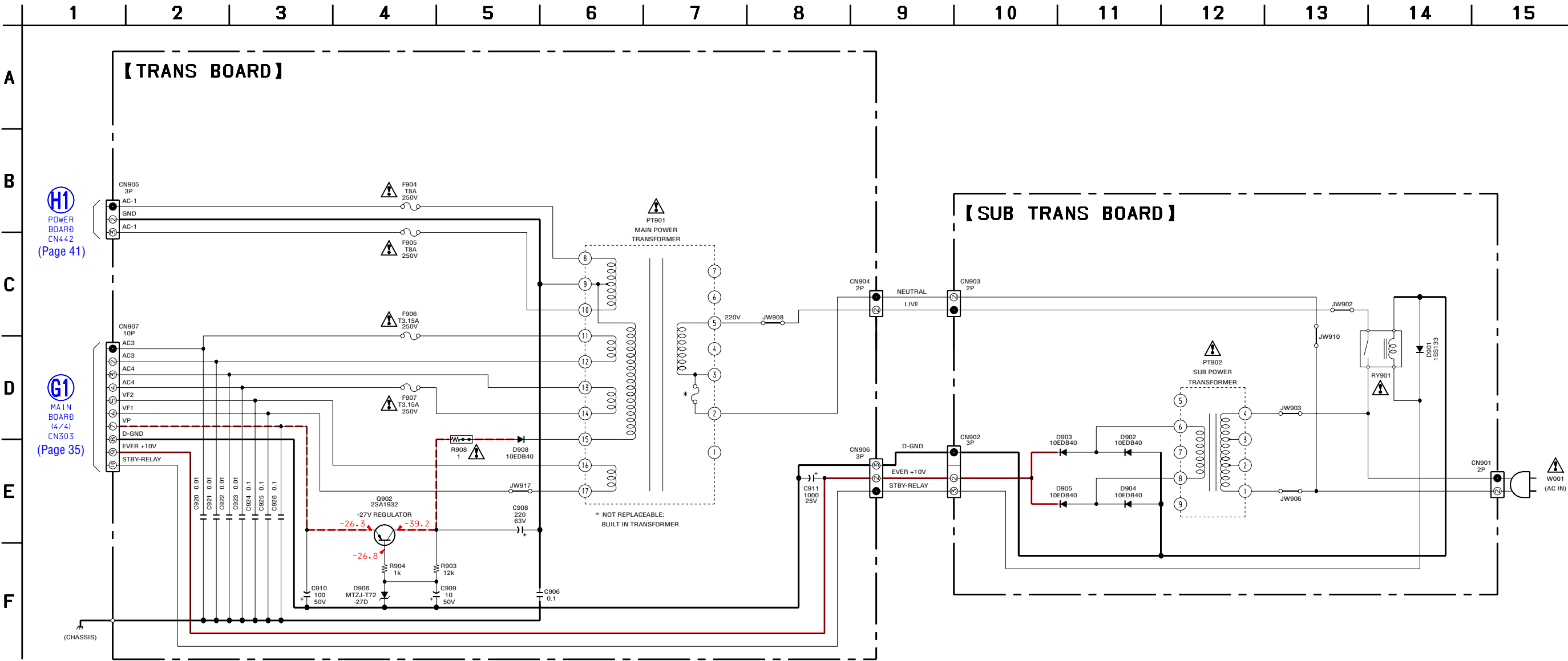
6-24. SCHEMATIC DIAGRAM – TRANS Section – (AEP, UK, CIS only)
