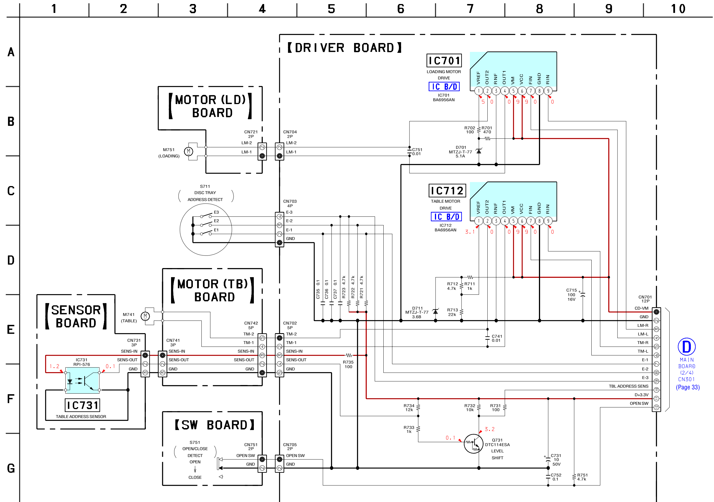
6-8. SCHEMATIC DIAGRAM – CHANGER Section – • See page 48 for IC Block Diagram.
