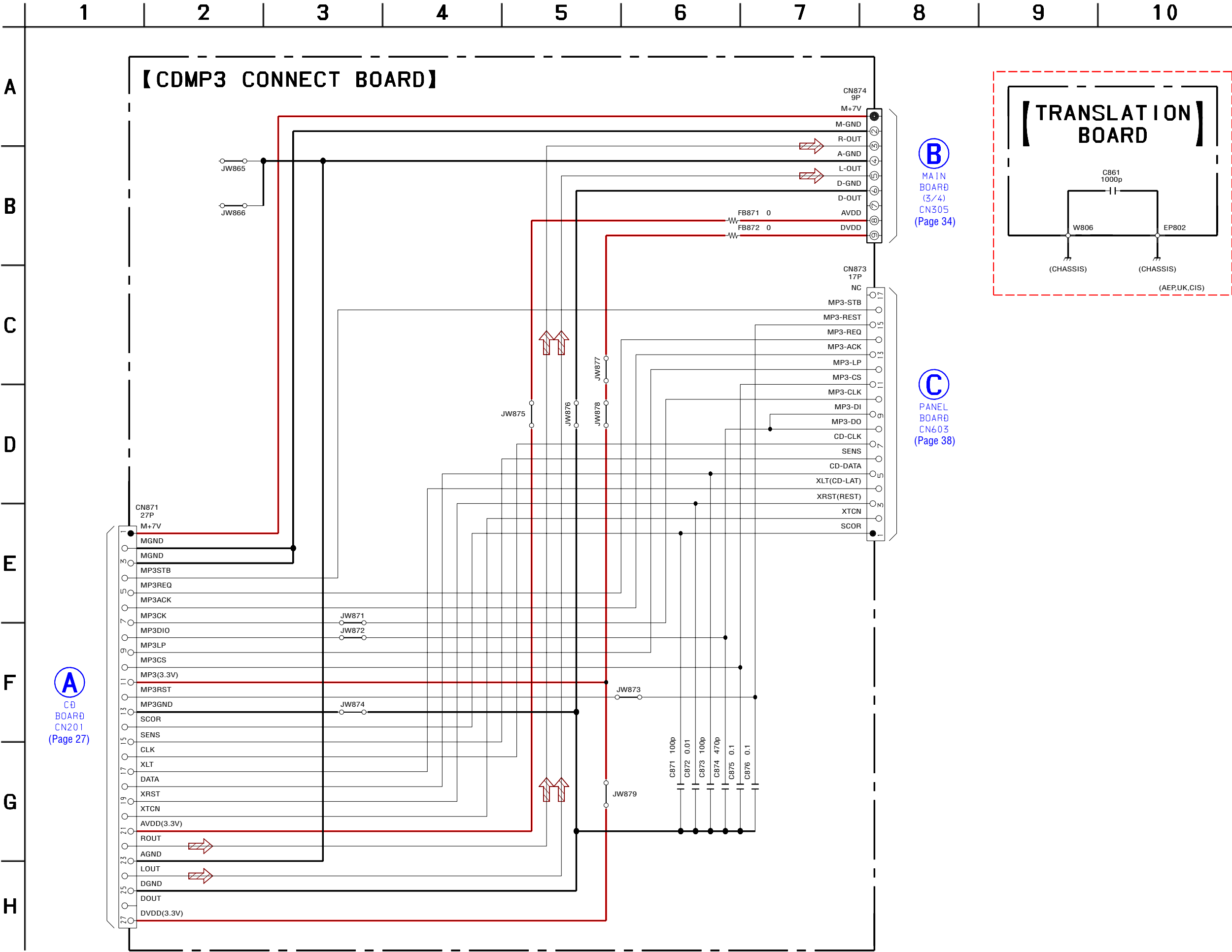
6-10. SCHEMATIC DIAGRAM – CDMP3 CONNECT/TRANSLATION Boards –
