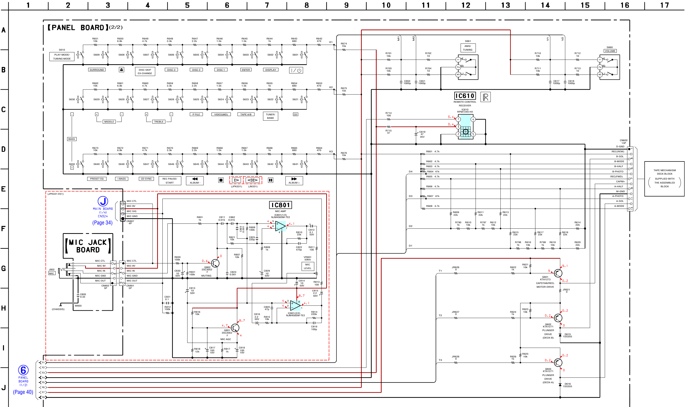
7-17. SCHEMATIC DIAGRAM – PANEL Section (2/2) –
