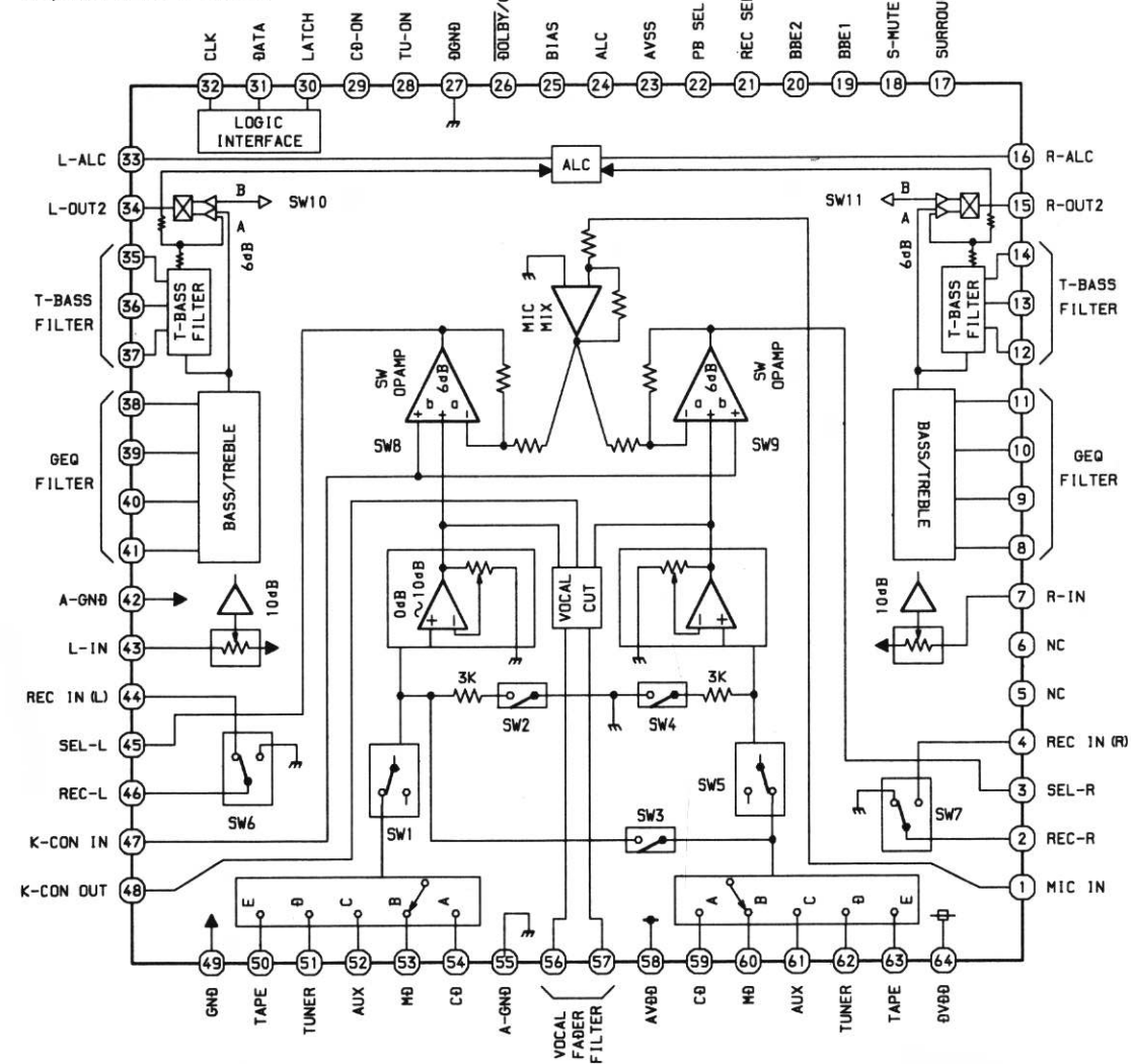
IC, M62445FP-600D
