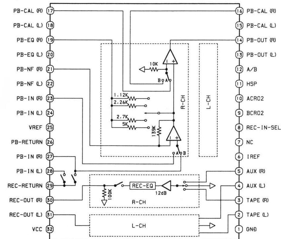
IC, BA7762AFS
