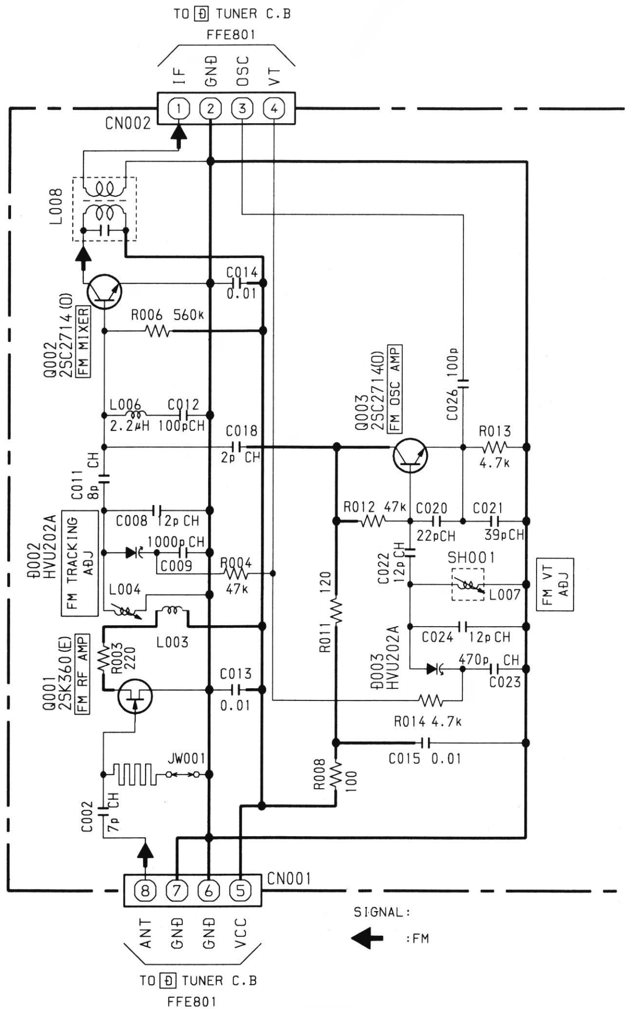
SCHEMATIC DIAGRAM - 9 (TUNER FRONT END)
