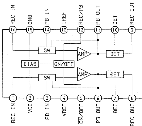
IC, HA12134A
