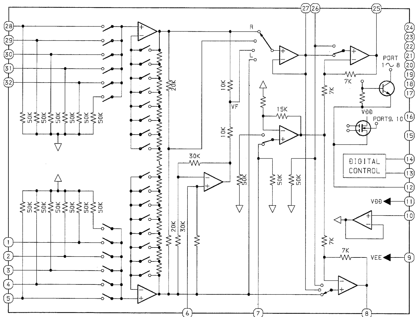
IC, BH3810FS
