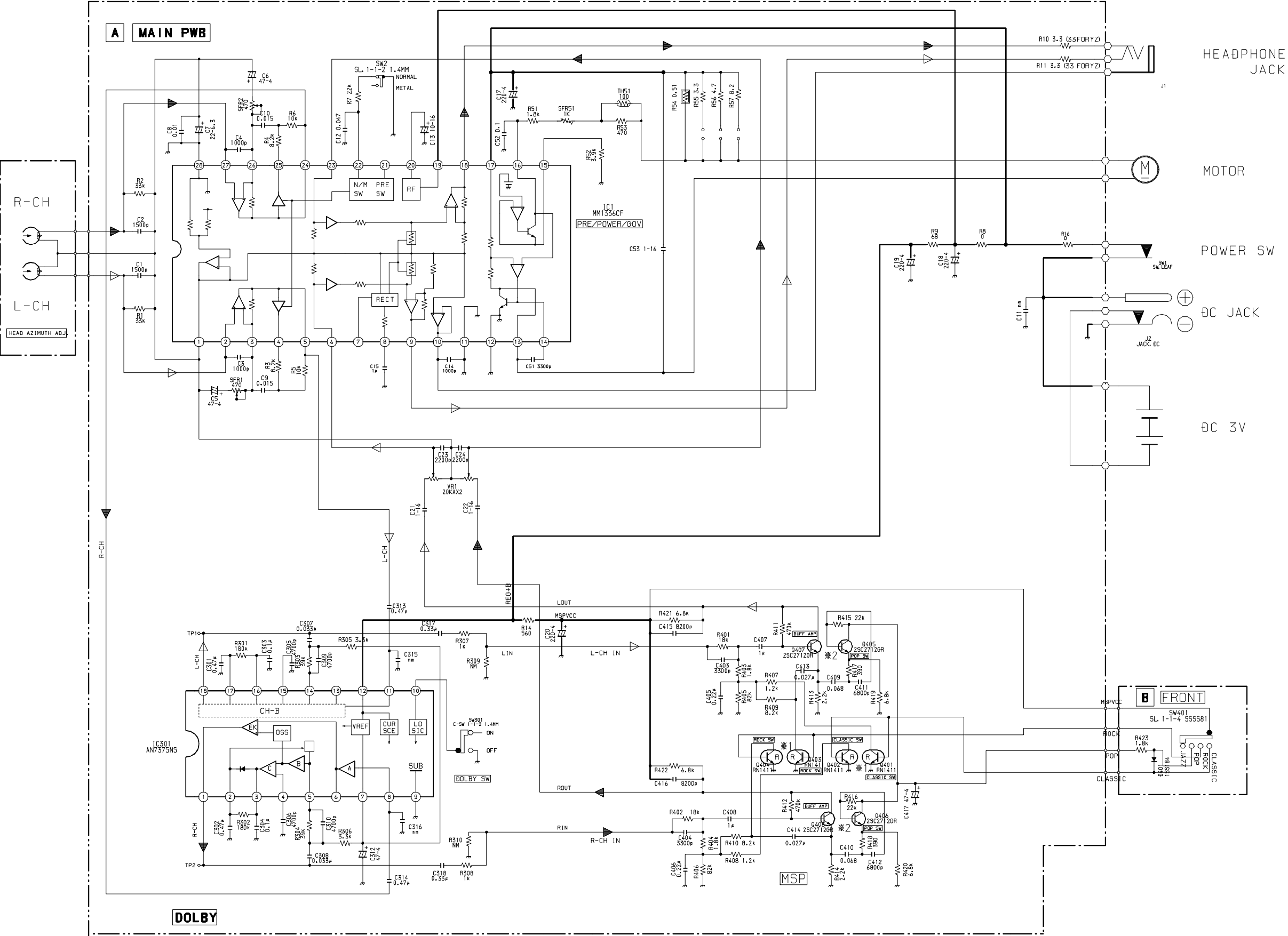
SCHEMATIC DIAGRAM
