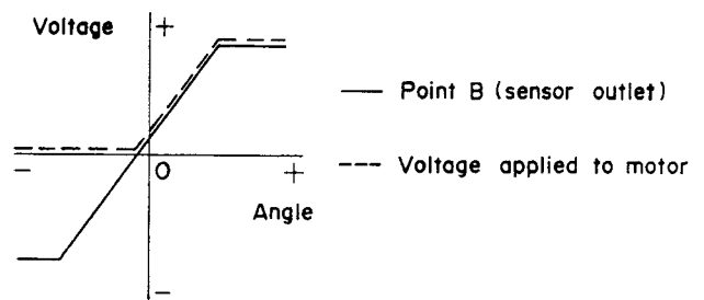
Fig. 5 Motor terminal waveform with electric governor
