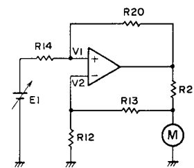
Fig. 3 Electric governor equivalent circuit
