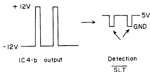
Fig. 16 Level conversion
