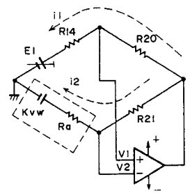
Fig. 4 Simplified equivalent circuit of electric governor
