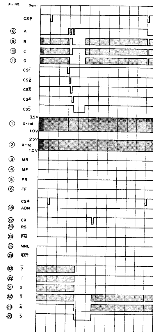
CPU(IC14) Timingchart
