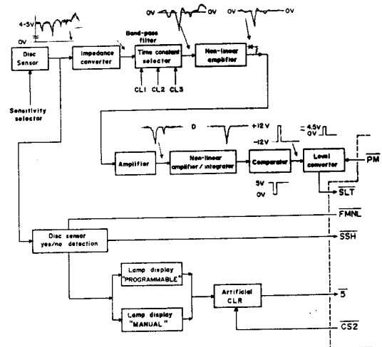
Fig. 11 Block diagram of disc sensor circuit
