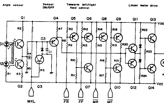
Fig. 6 Linear motor control and drive circuit
