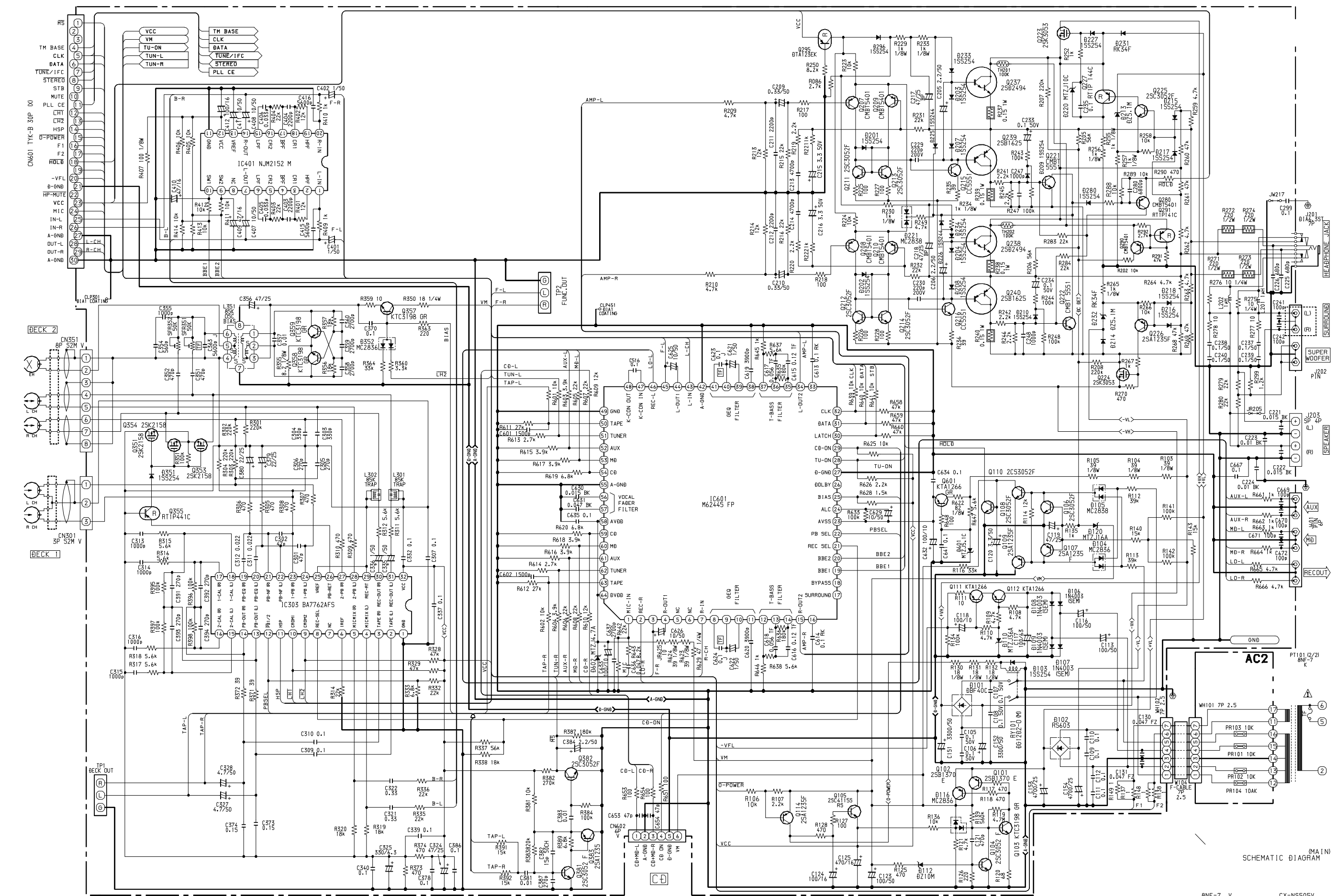
SCHEMATIC DIAGRAM – 1 (505V : MAIN)
