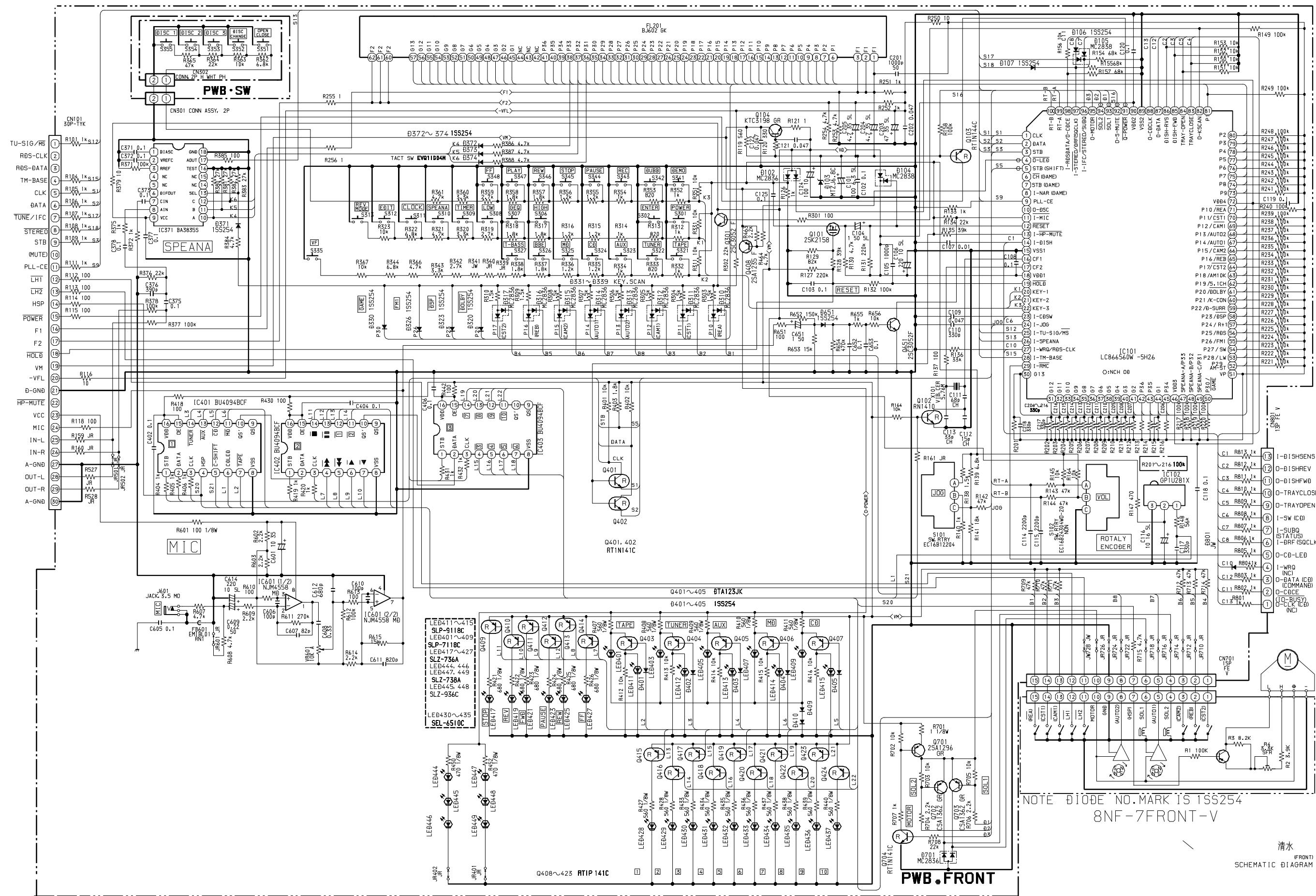
SCHEMATIC DIAGRAM – 5 (505V : FRONT)
