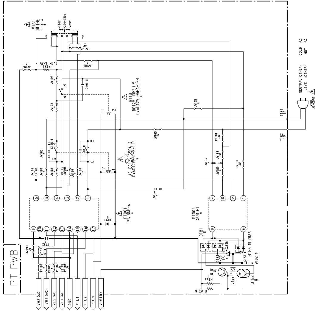
SCHEMATIC DIAGRAM - 2 (MAIN 2/2: PT)
