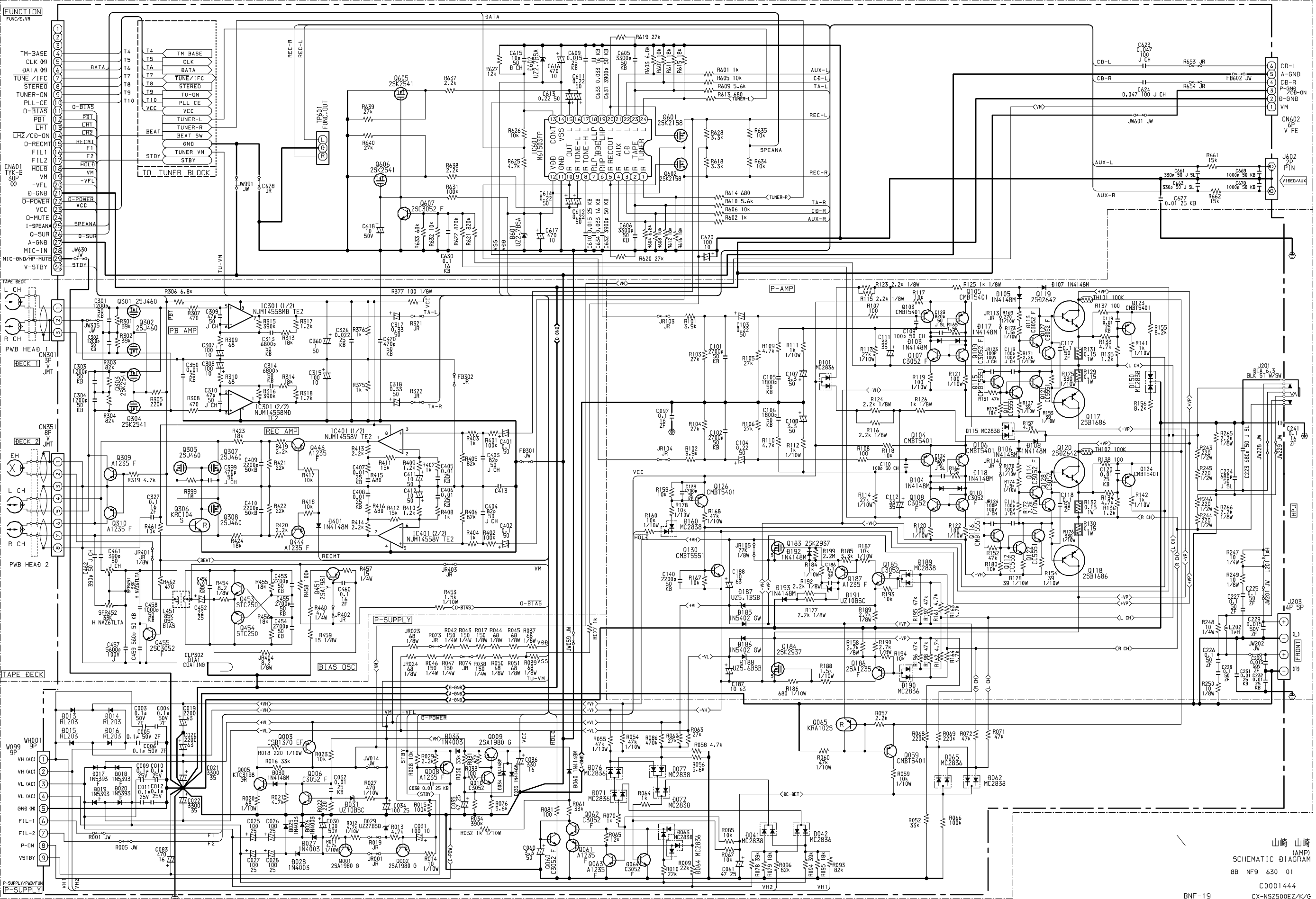
SCHEMATIC DIAGRAM-4 (MAIN) <EZ>
