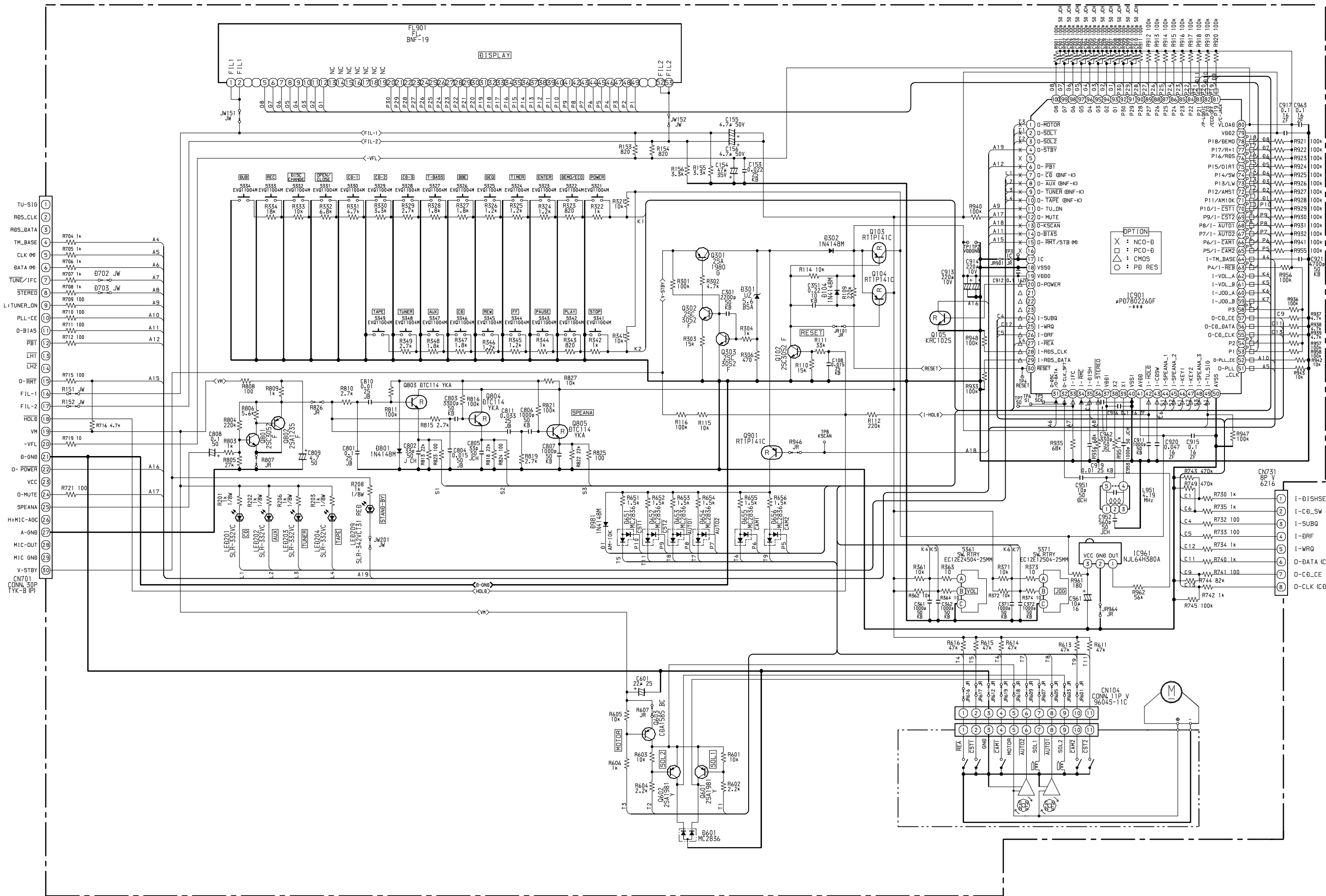
SCHEMATIC DIAGRAM – 8 (FRONT) <U>
