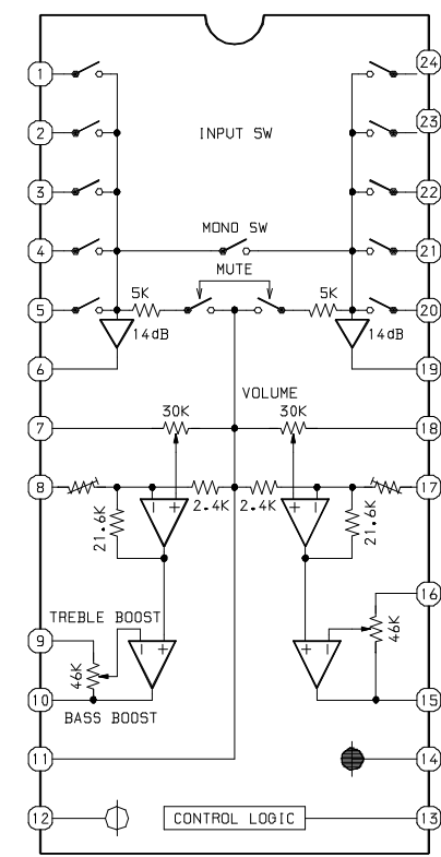
IC BLOCK DIAGRAM IC,M62495AFP
