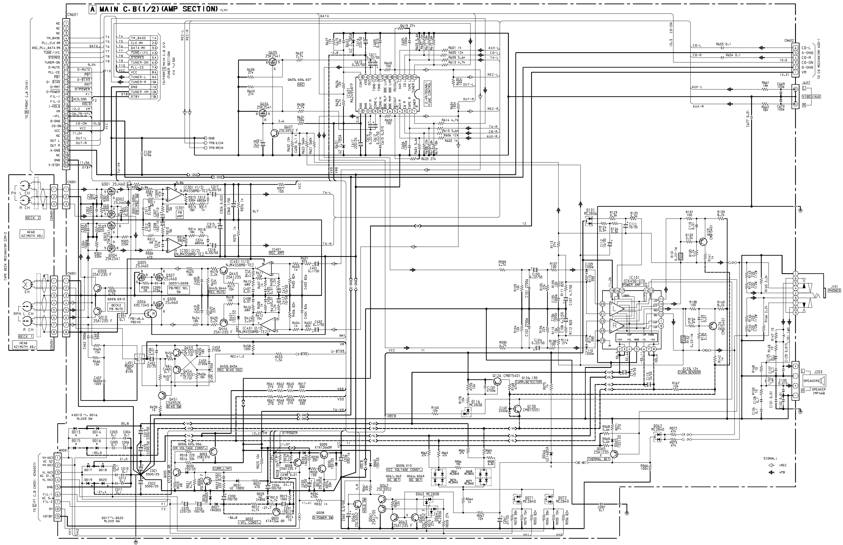
SCHEMATIC DIAGRAM – 3 (MAIN 1 / 2 : AMP SECTION)<LH>
