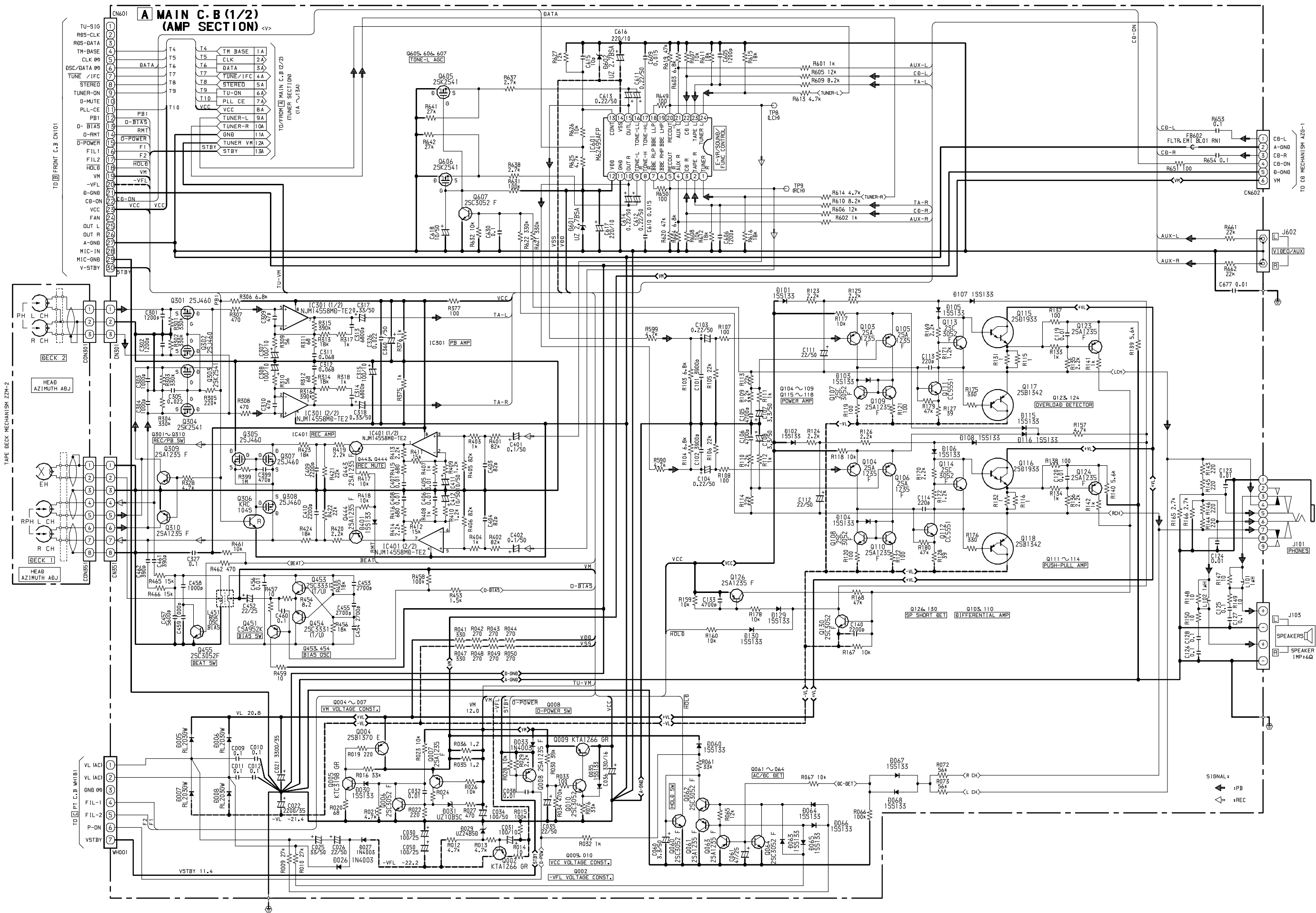
SCHEMATIC DIAGRAM – 5 (MAIN 1 / 2 : AMP SECTION)<V>
