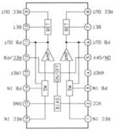
IC, HA12134A
