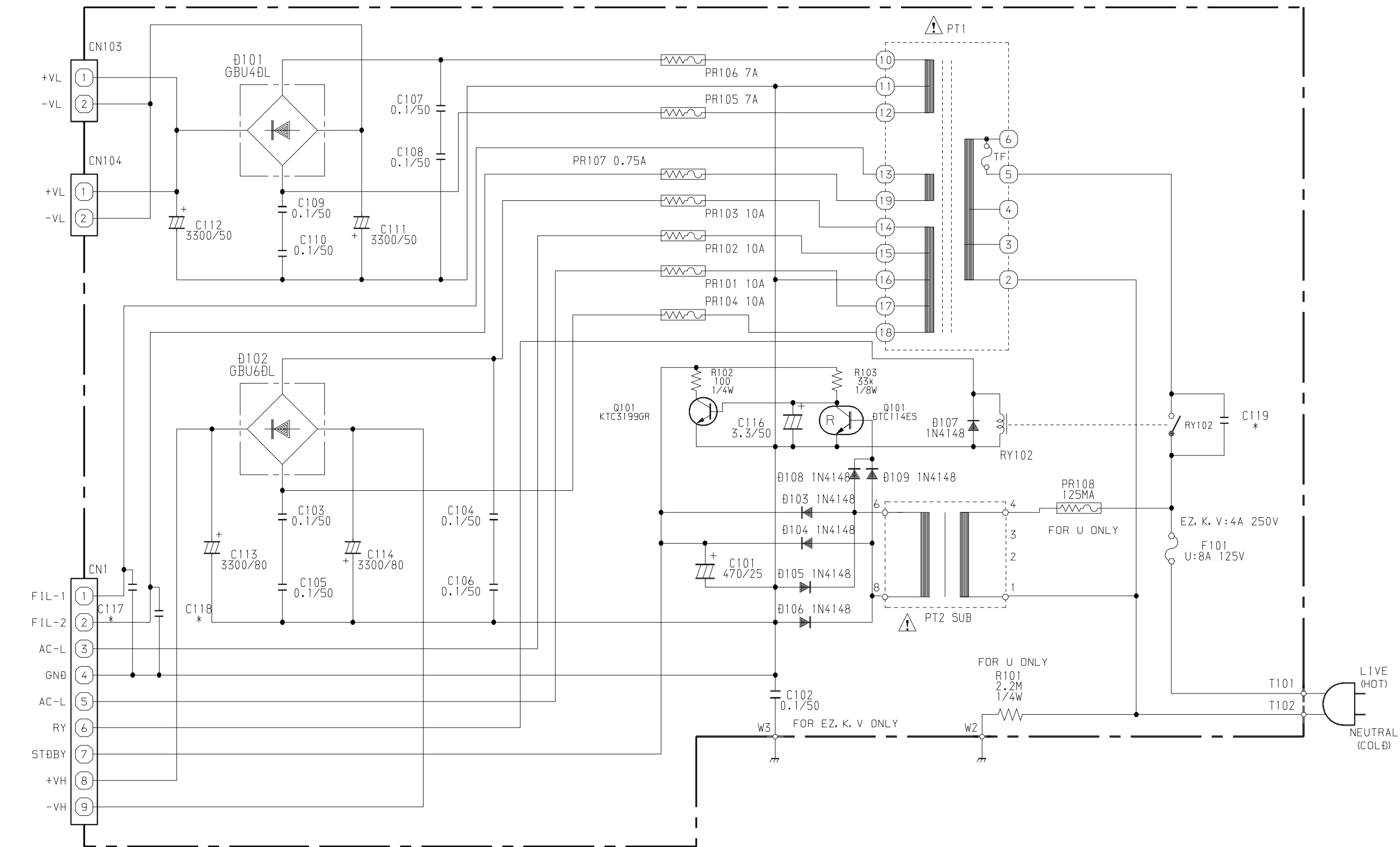
SCHEMATIC -PT
