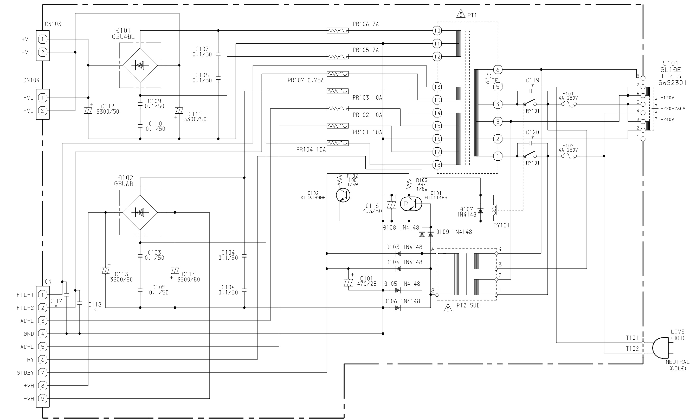
SCHEMATIC - PT
