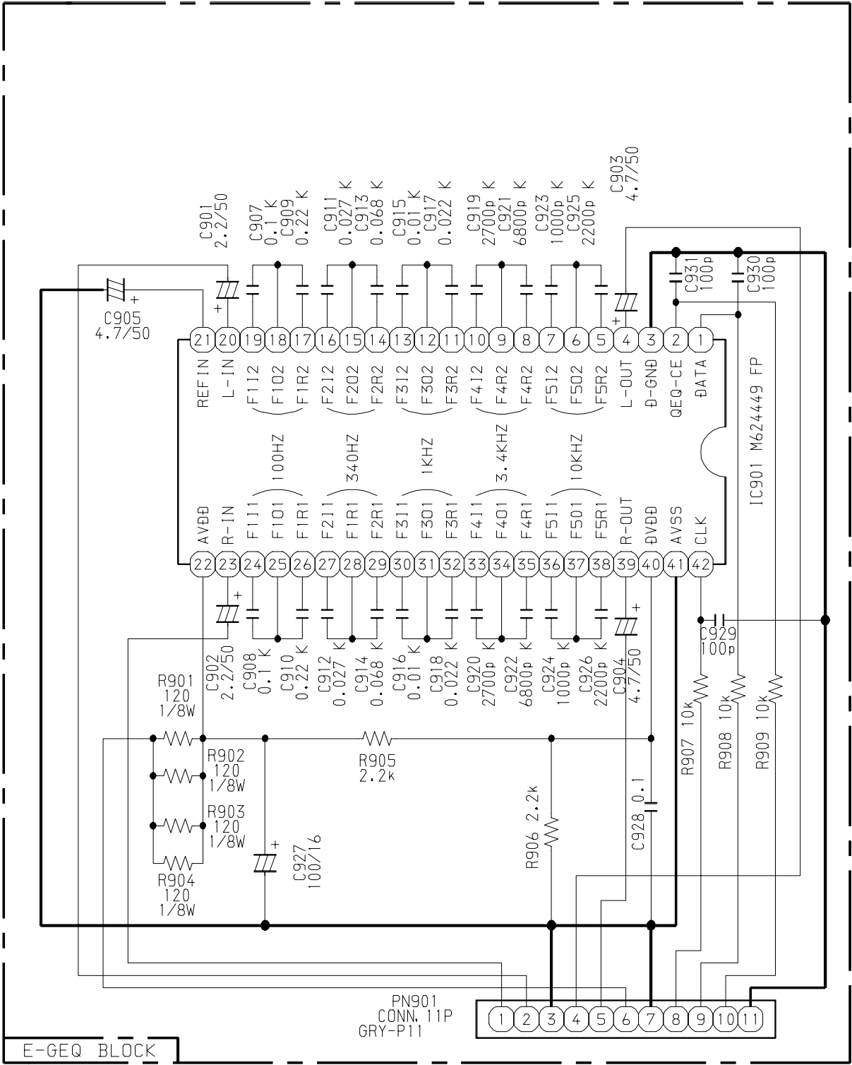
SCHEMATIC DIAGRAM – 3 (MAIN 3/3 · F7 K)
