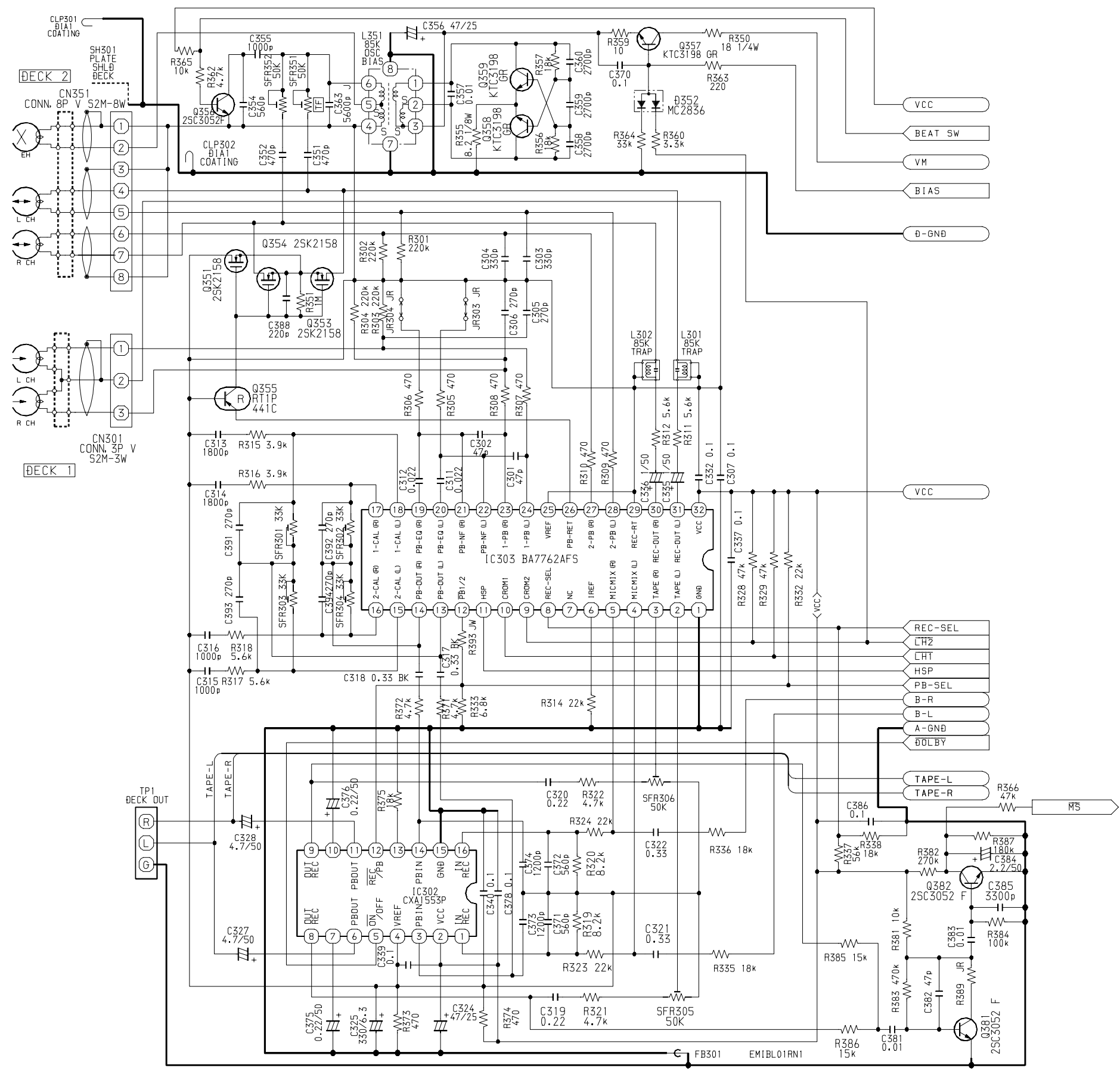
SCHEMATIC DIAGRAM - 2 (MAIN 2/3 · F7 K)
