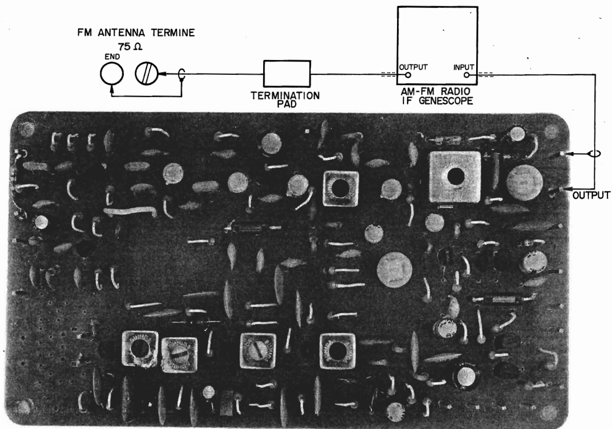
Fig. 7 INSTRUMENT CONNECTIONS
