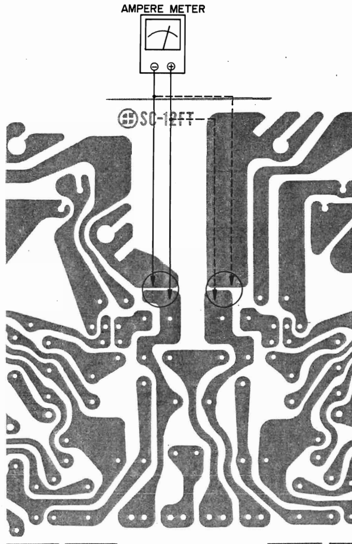
○ Indicates Soldering Points
