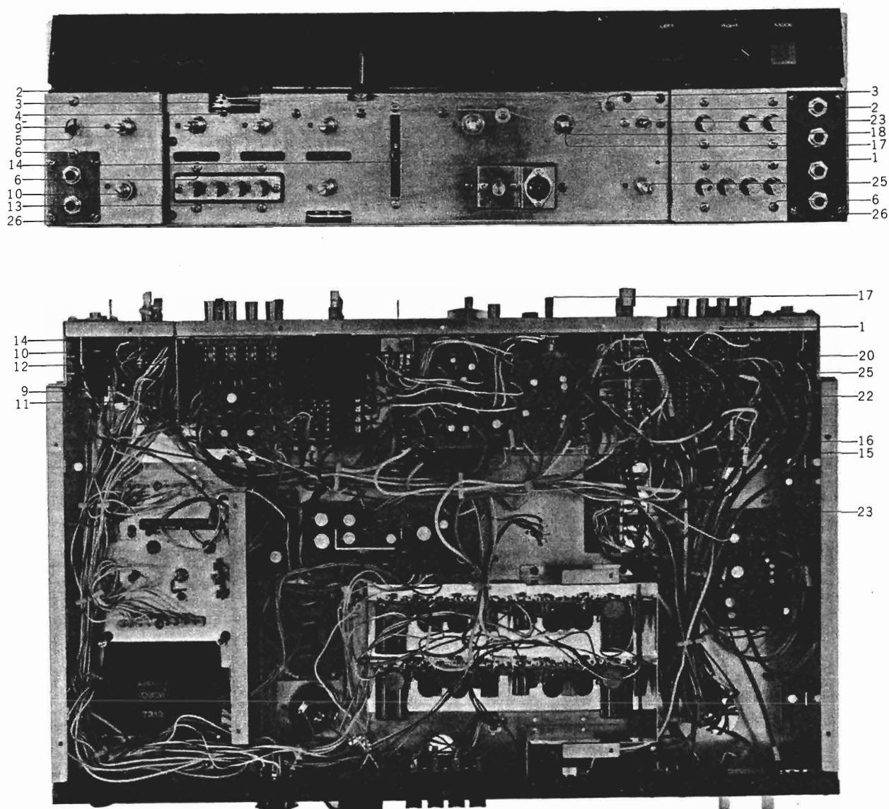
FIG. 19 PHOTO OF FRONT CHASSIS BLOCK
