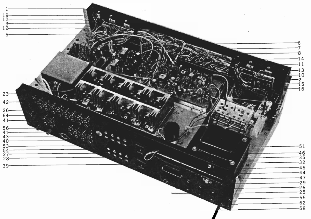
FIG. 20 PHOTO OF SCALE MT. PLATE/REAR PANEL BLOCK
