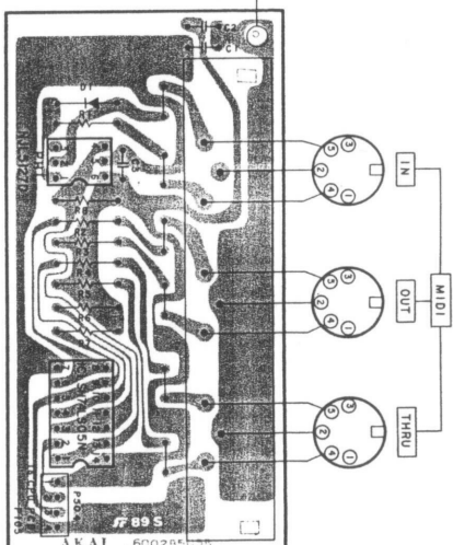
MIDI JACK PCB L6002B505B
