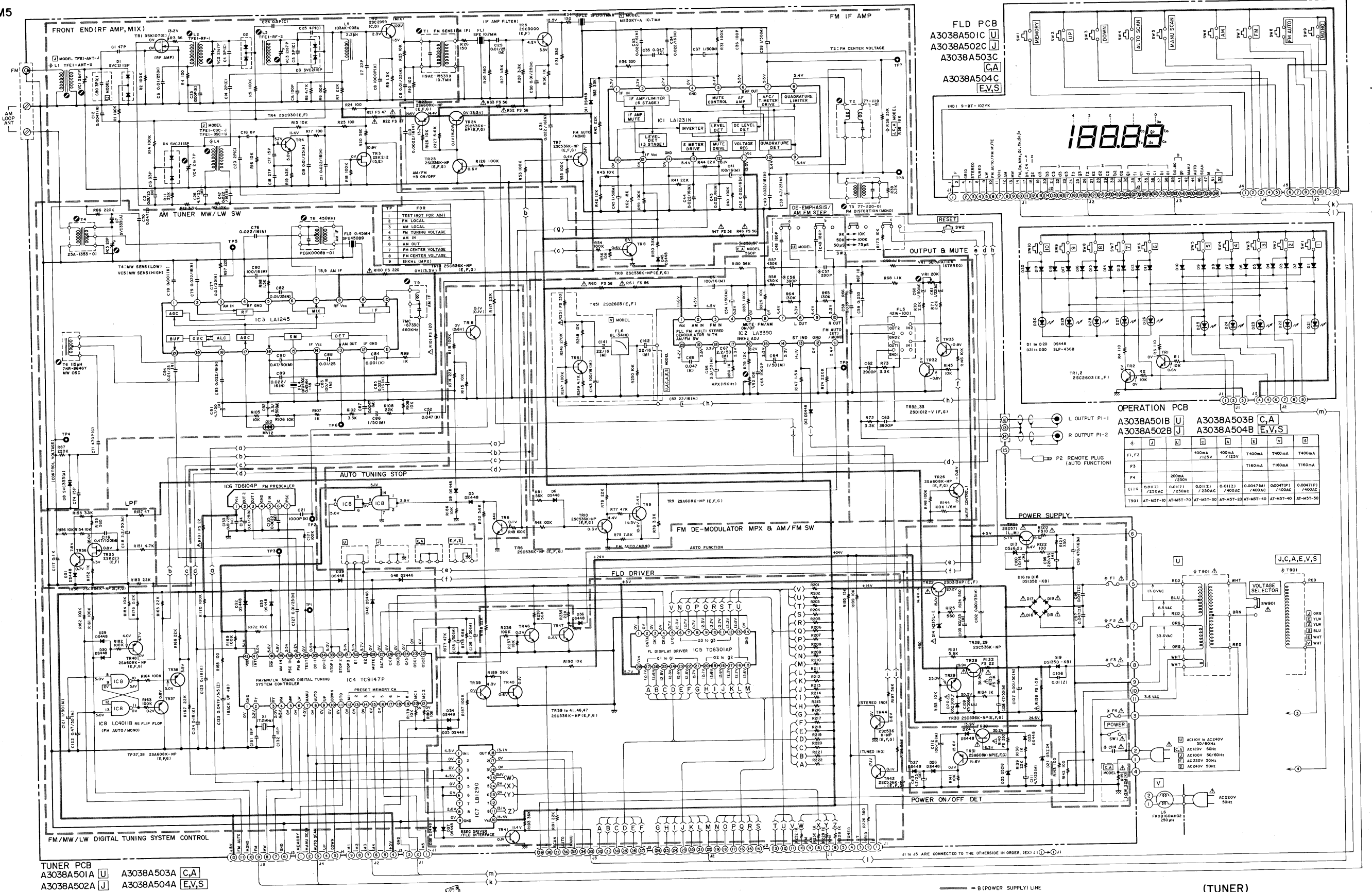
(TUNER) AT-M5 SCHEMATIC DIAGRAM No. 830212A
