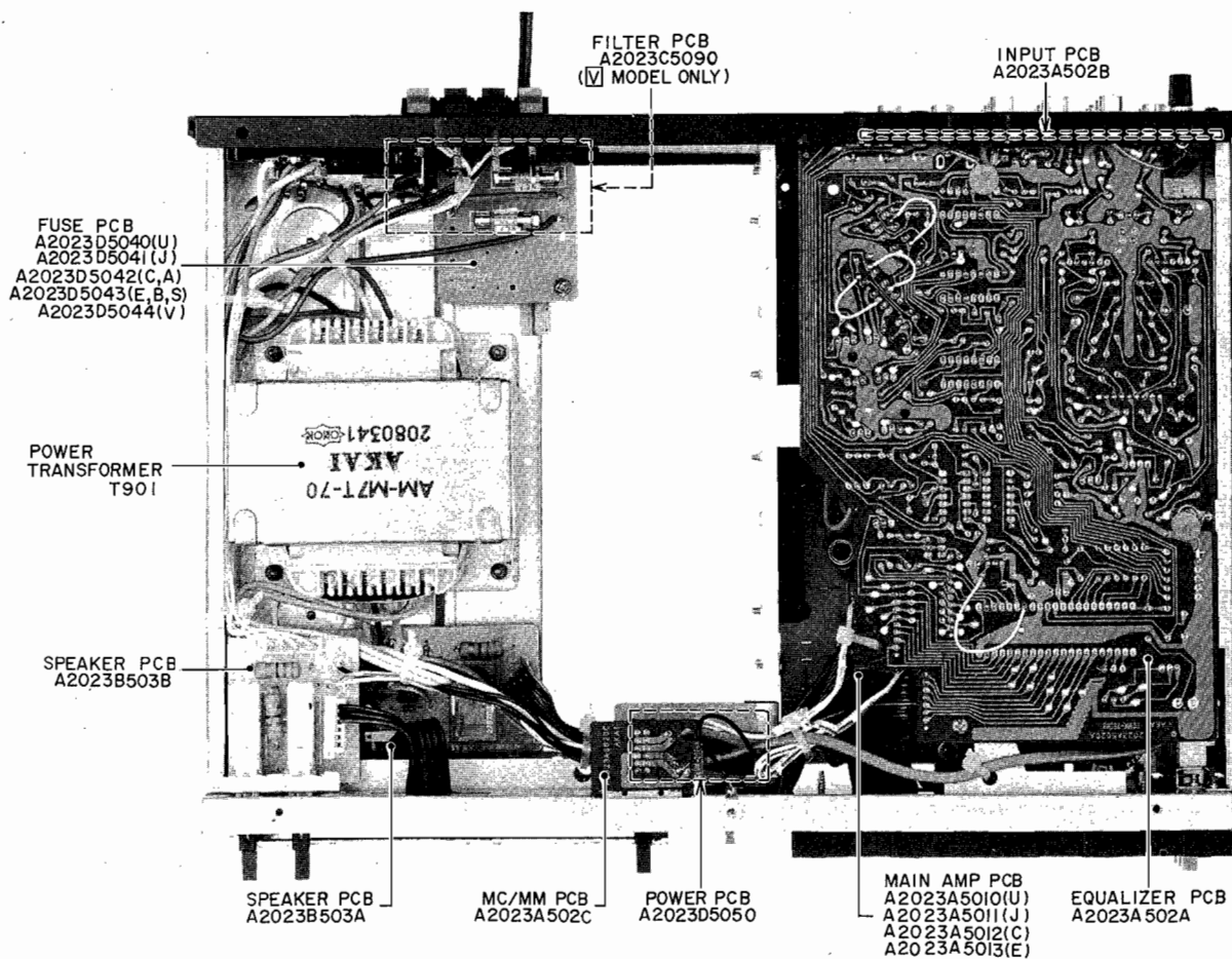
Fig. 4-4 Top View
