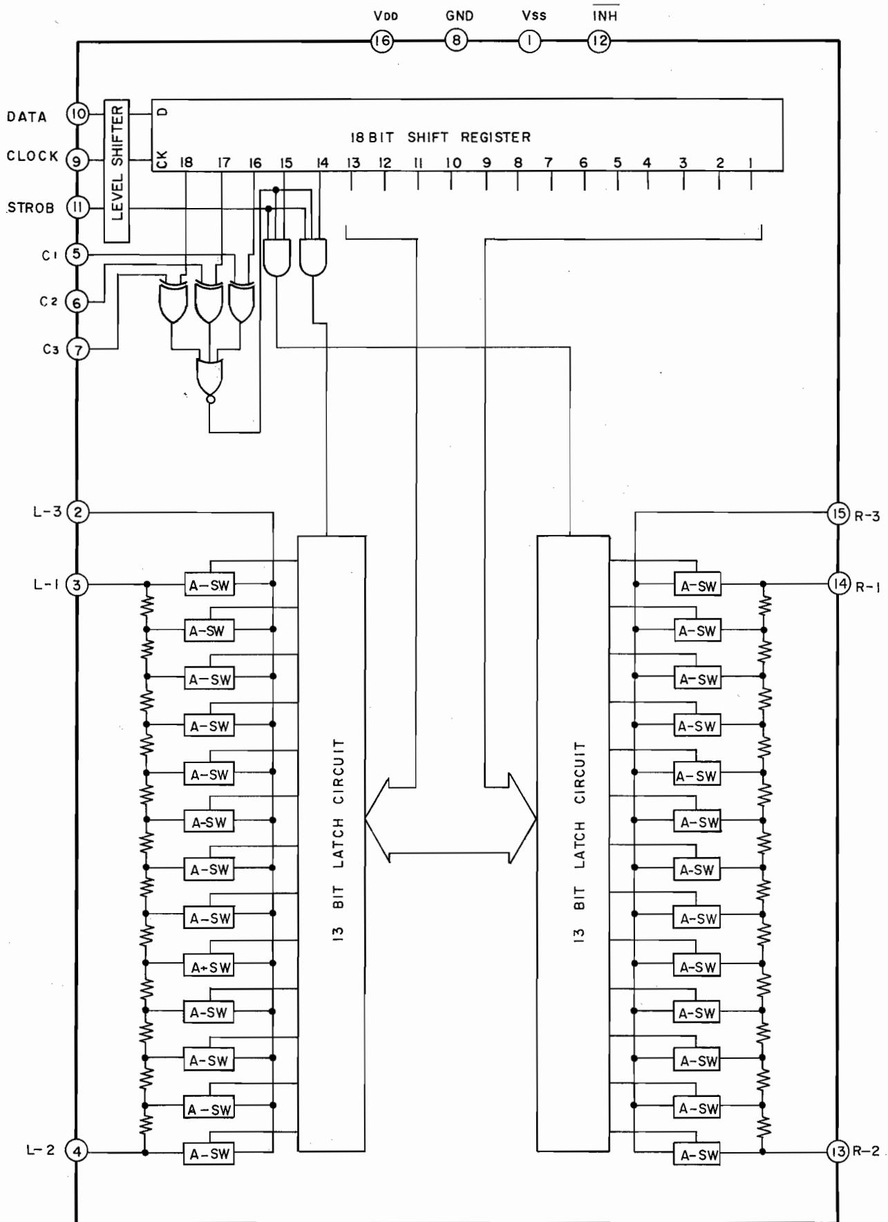
SCHEMATIC DIAGRAM AT-M5/L AM-M5/M7
