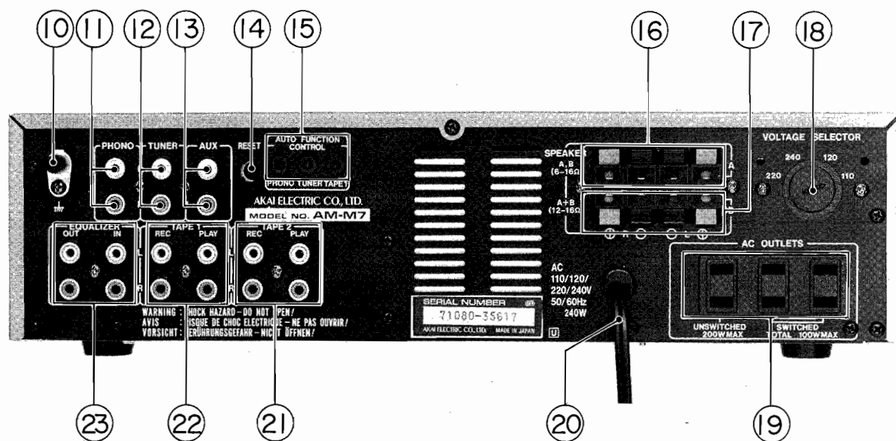
Fig. 3-4 Rear View
