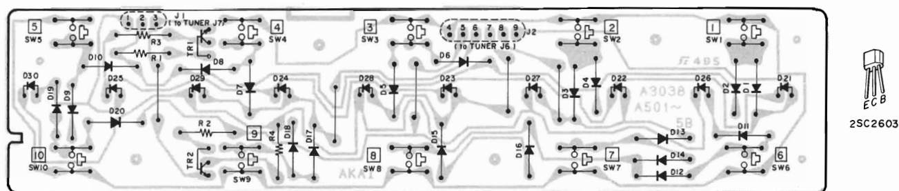
OPERATION PCB A3038A501B to 5B (ALL MODELS)
