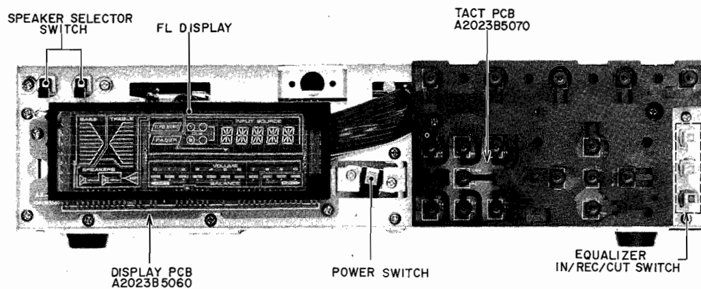
Fig. 4-1 Front View
