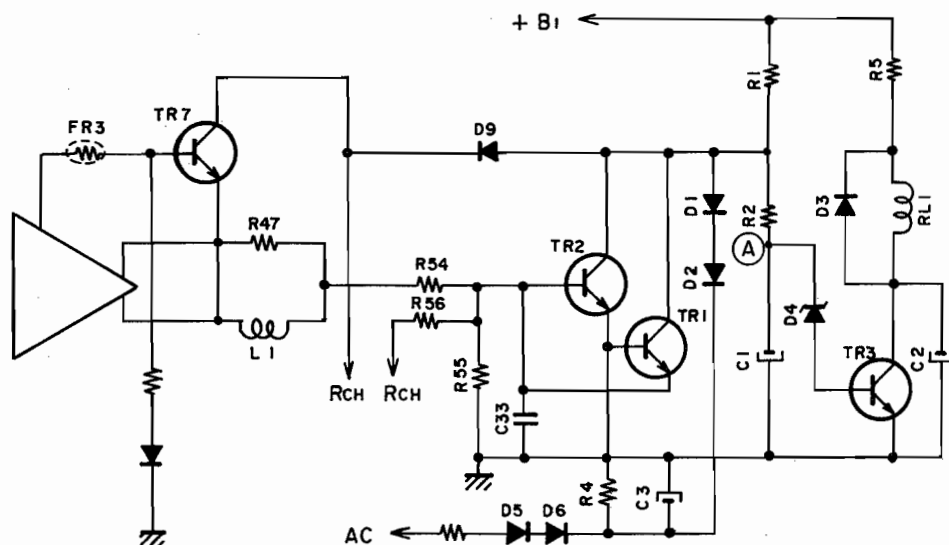
Fig. 3-1 Protection Circuit
