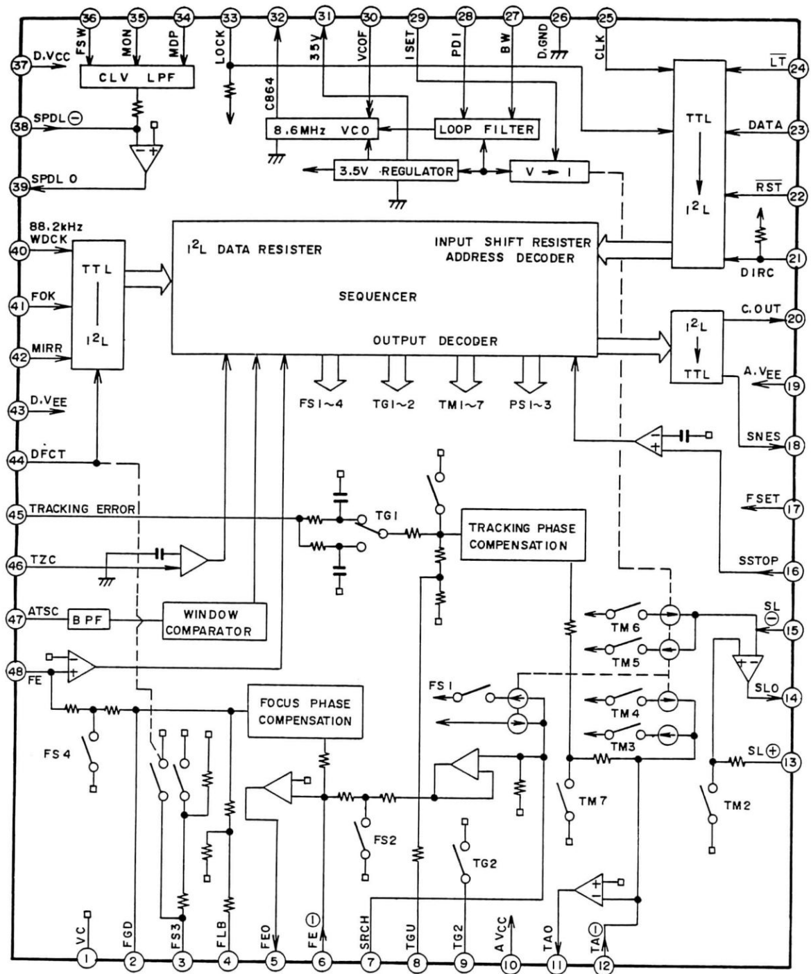
CXA 1082A
