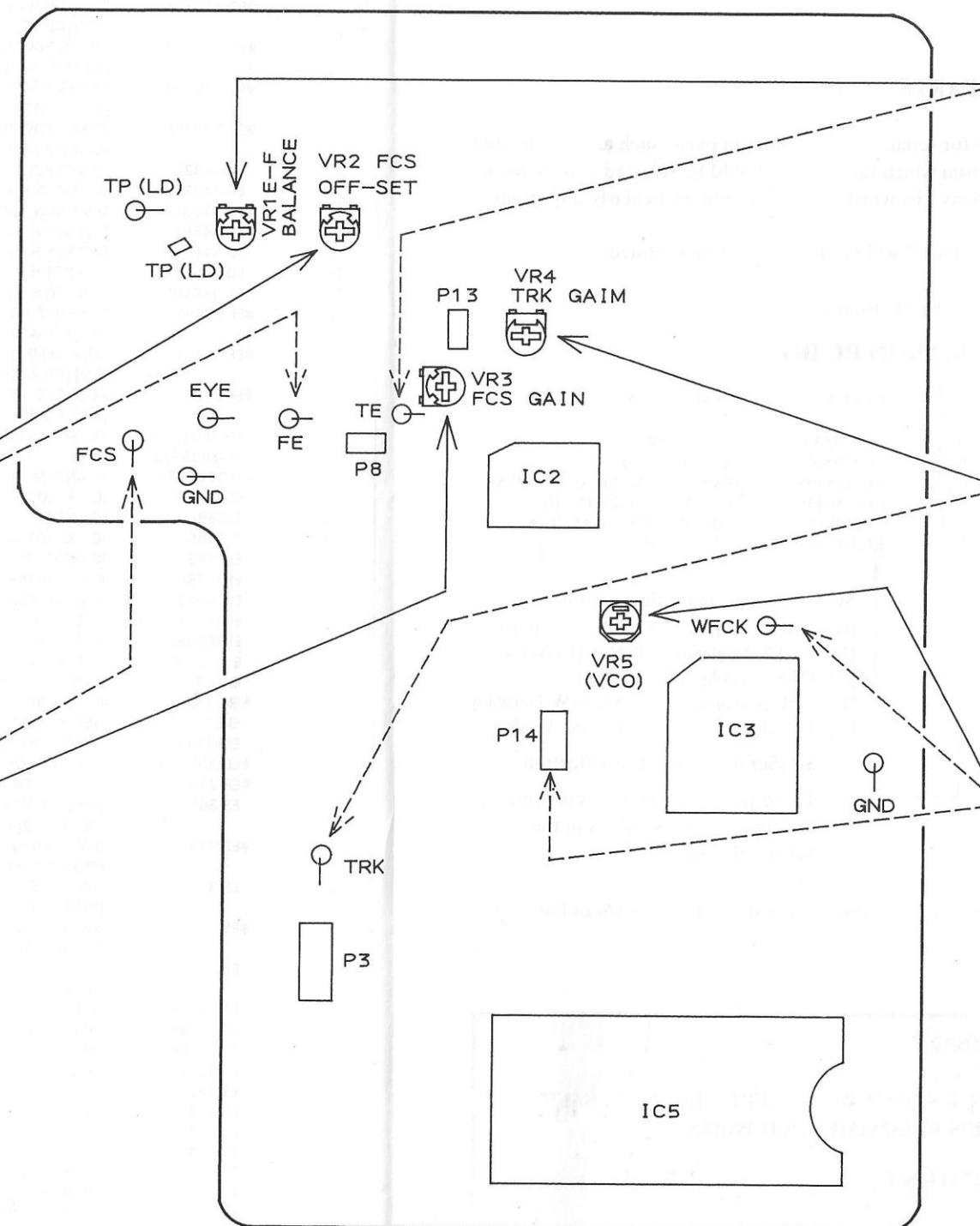
MAIN PCB
