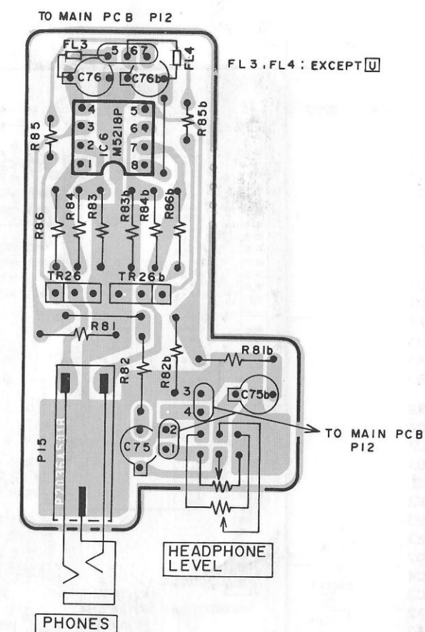
HEADPHONE PCB (J3) P2036A501B
