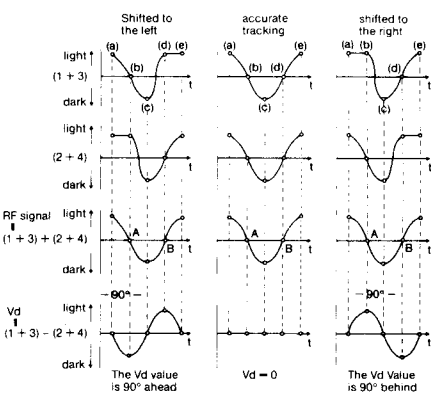
Fig. 6-5 Wave Patterns for Each Case
