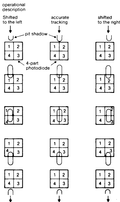
Fig. 6-4 Tracking Detection
