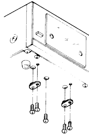
Fig. 1-1 Transit Screws
