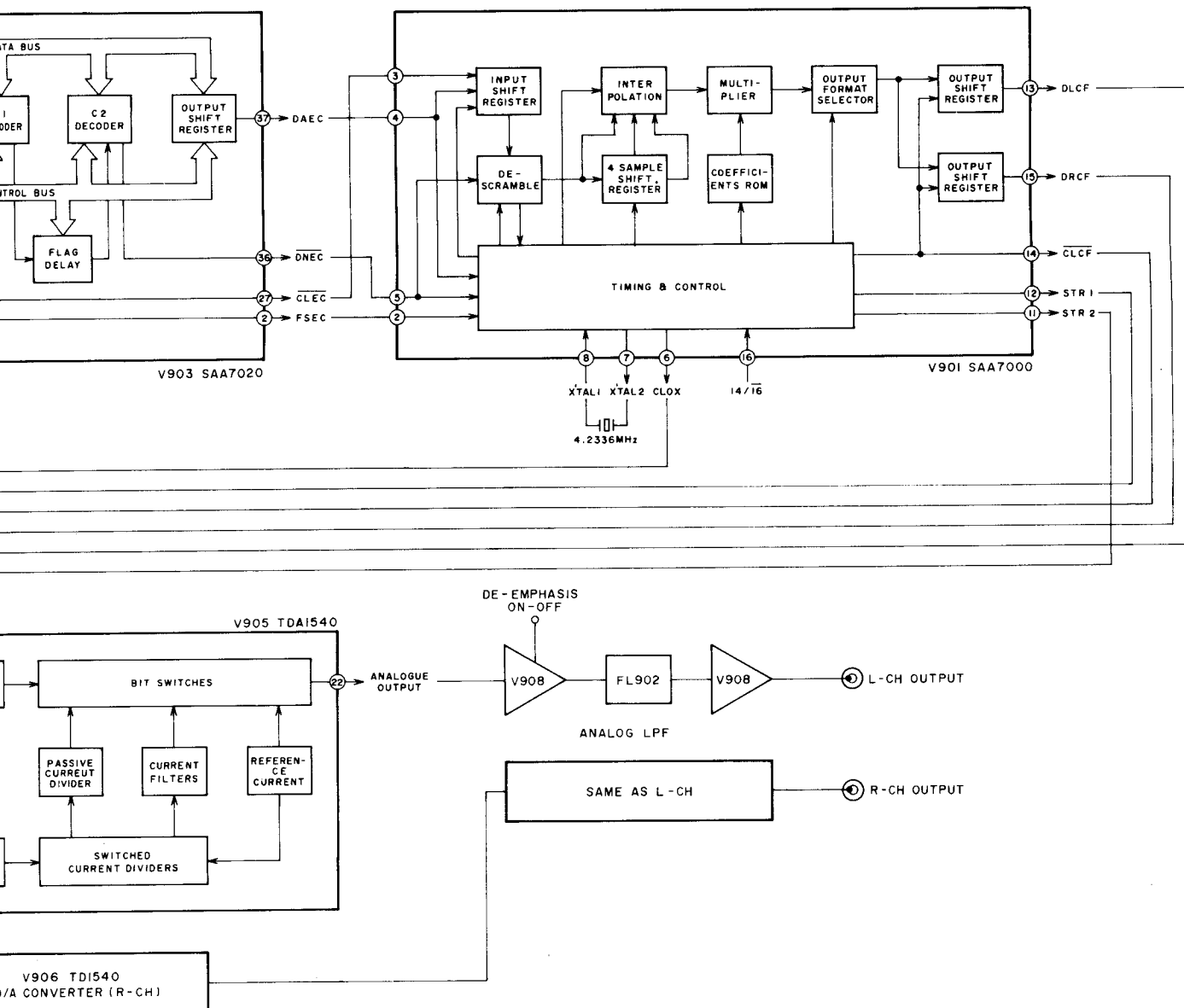
Fig. 6-2 Signal Process of C.D Block Diagram
