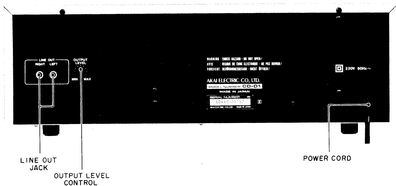
Fig. 4-2 Rear View
