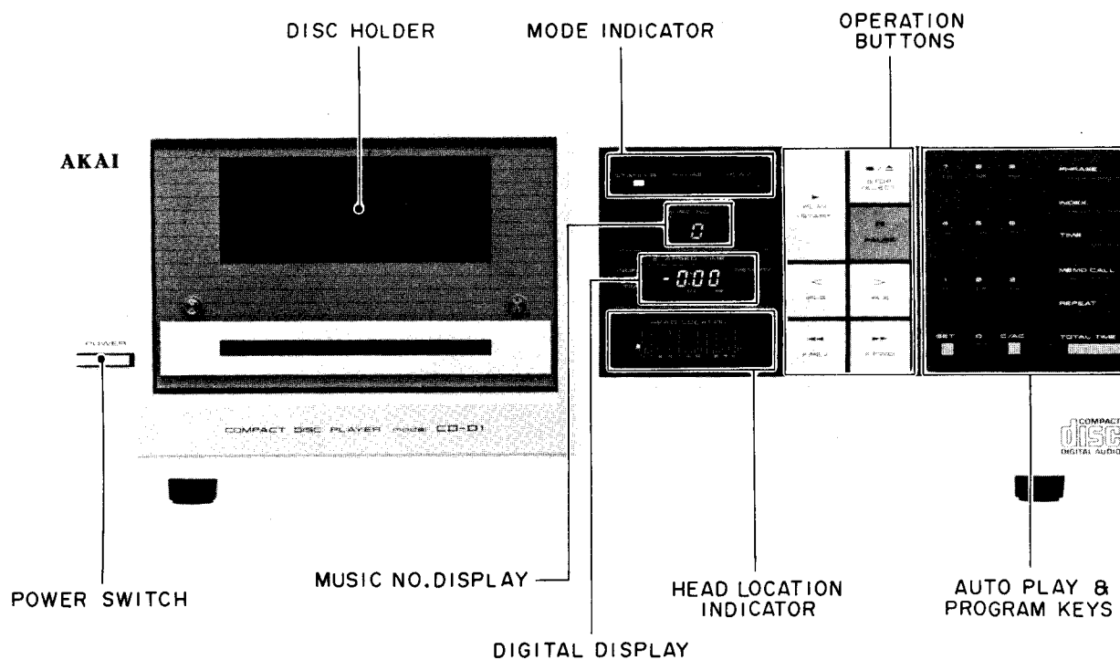
Fig. 4-1 Front View
