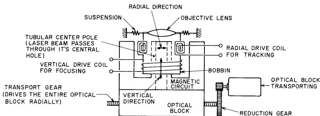
Fig. 6-8 Structure of Focusing Screw
