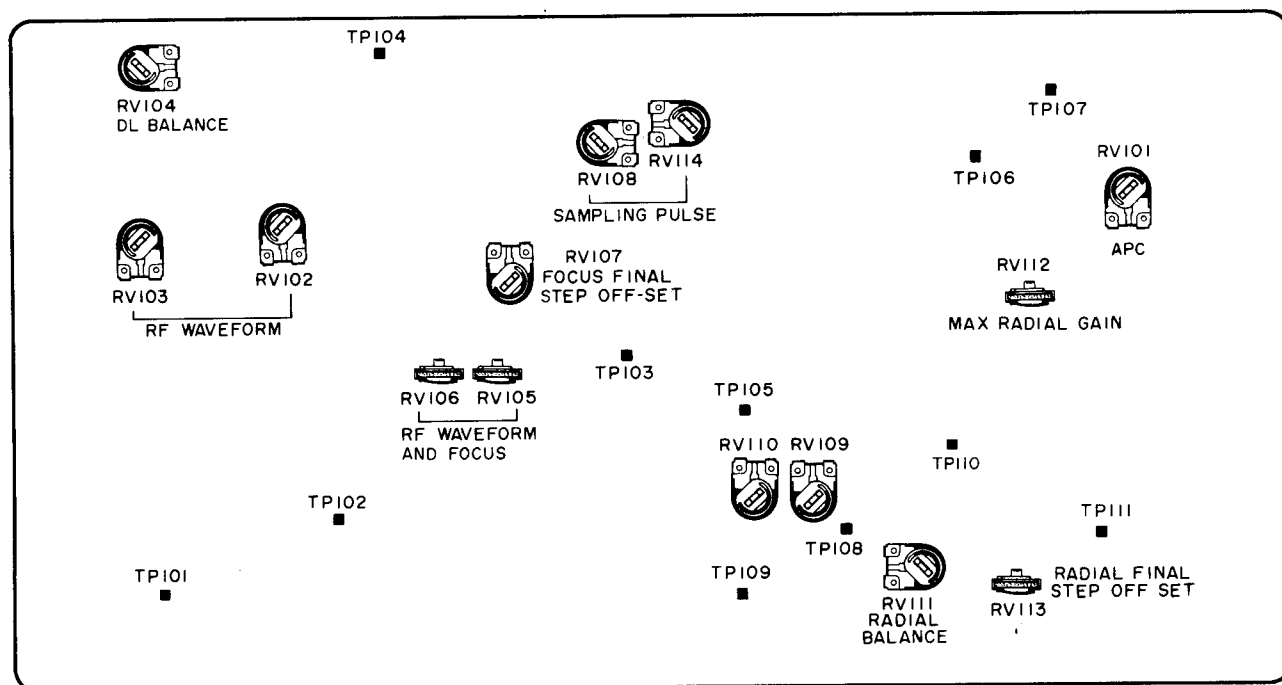
Fig. 7-1 Servo P.C Board Adjustment Points
