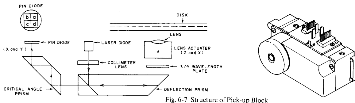
Fig. 6-7 Structure of Pick-up Block
