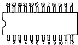
U904: SAA7030 (M4550)
