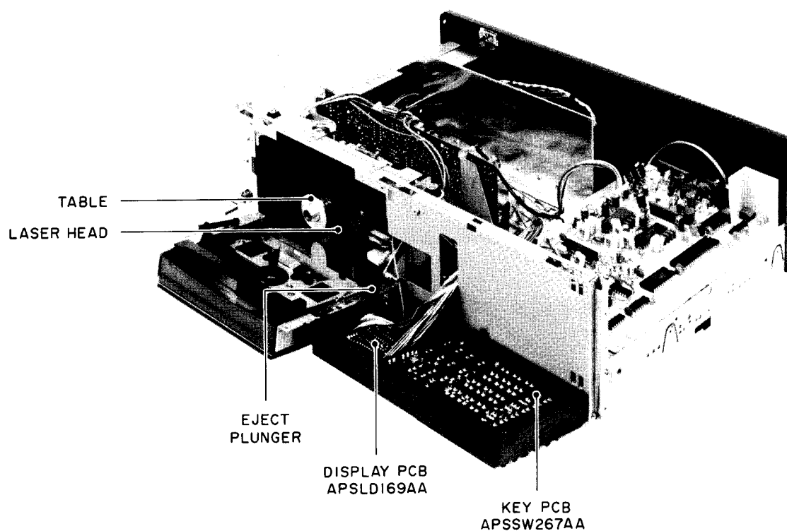
Fig. 5-2 Front View
