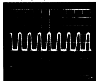
Pin 10 (0.2 \mu sec/div. 0.2V/div.)
