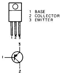
Q505: 2SA768 Q507
