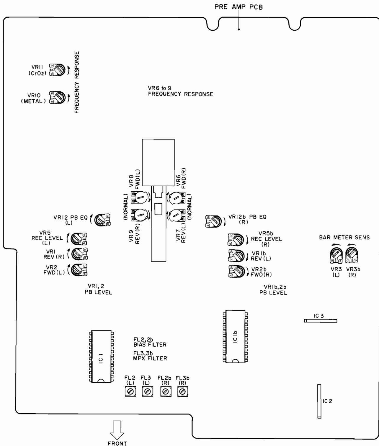
Fig. 19 Amplifier Adjustment (CS-F39R)
