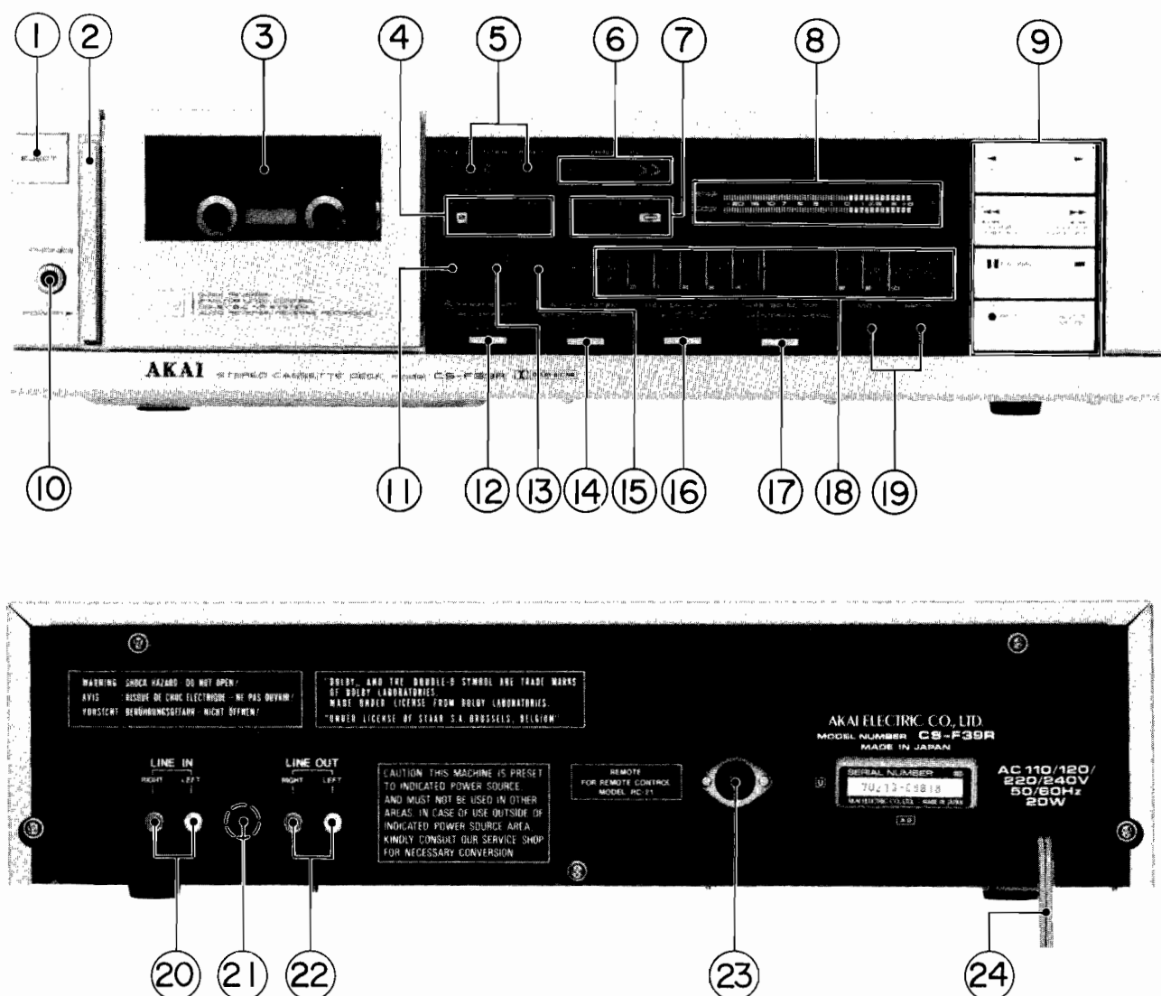
Fig. 2 Controls
