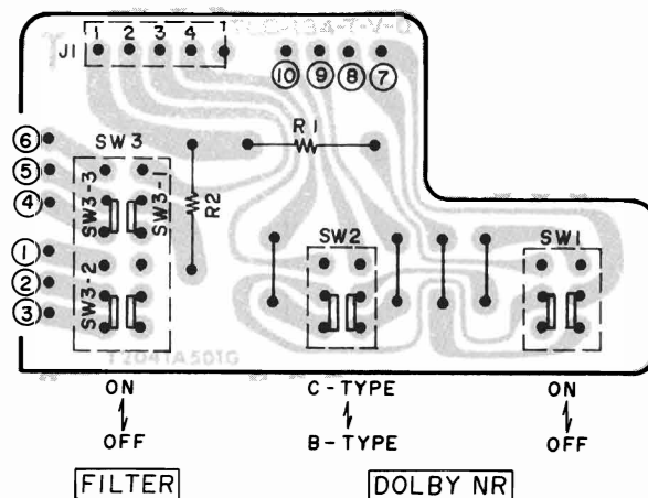
DOLBY SWITCH PCB T2041A501G
