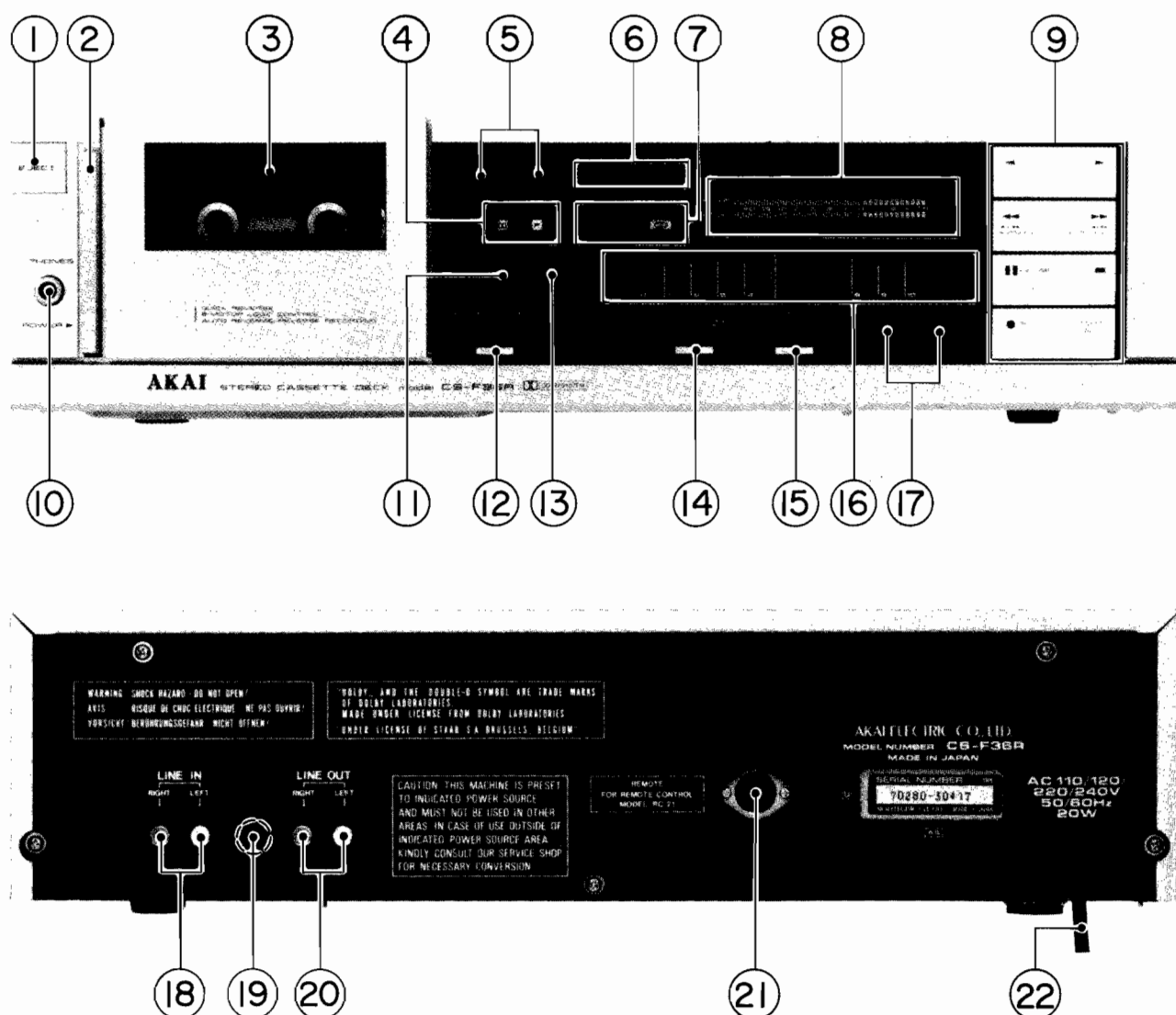
Fig. 1 Controls
