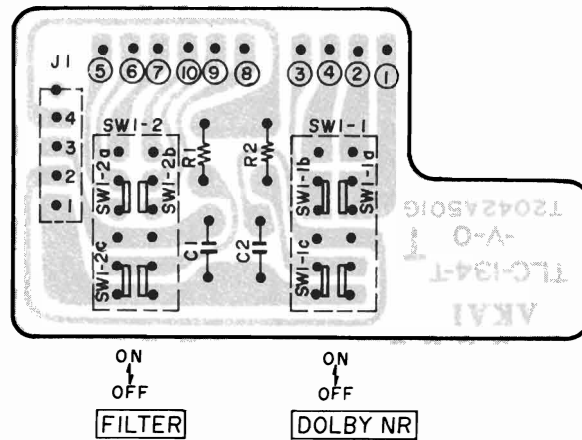
DOLBY SWITCH PCB T2042A501G
