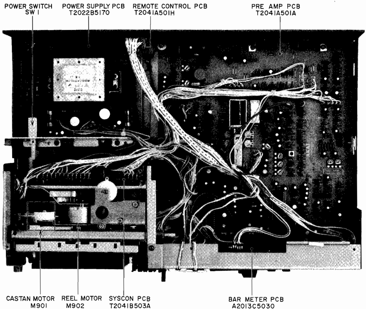
Fig. 6 Top View
