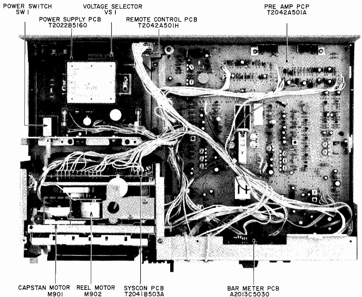
Fig. 4 Top View
