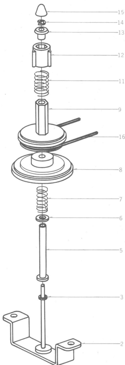
FIG. 3 ILLUSTRATION OF TAKE-UP TABLE BLOCK
