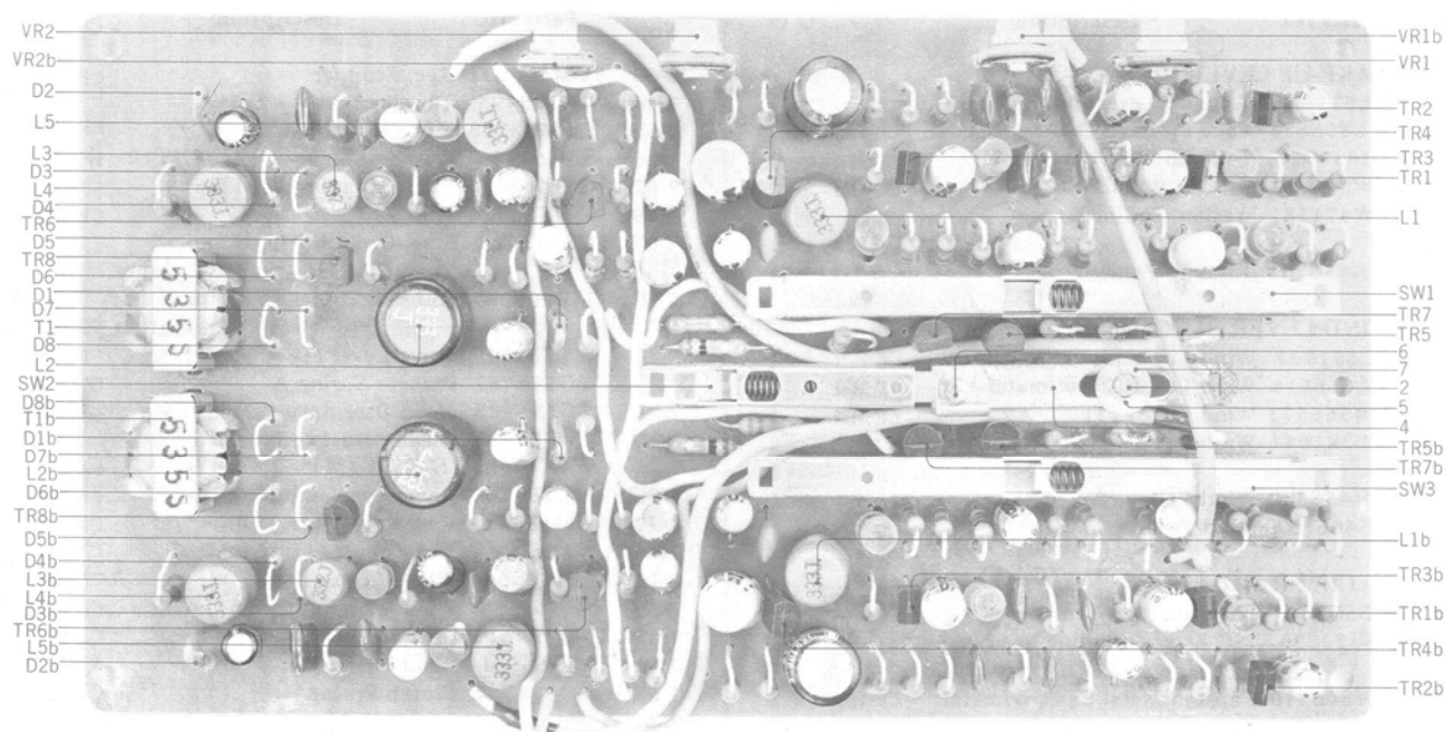
FIG. 8 PHOTO OF PRE-AMP. P.C. BOARD (CP-5002) BLOCK
