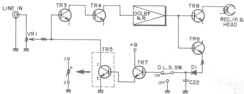
Fig. 55 O.L.S. Block Diagram
