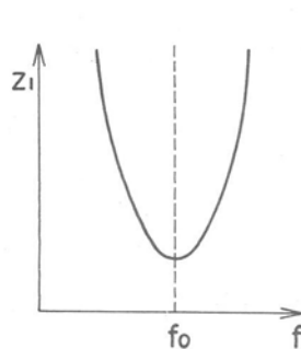
Fig. 53 B.P.F./Impedance characteristics
