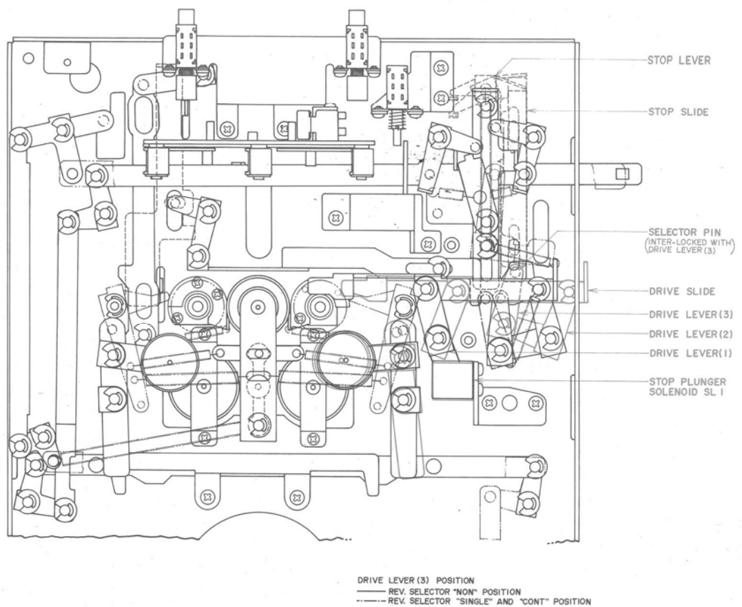
Fig. 30 Reverse Selector : NON → From FWD to STOP Mode
