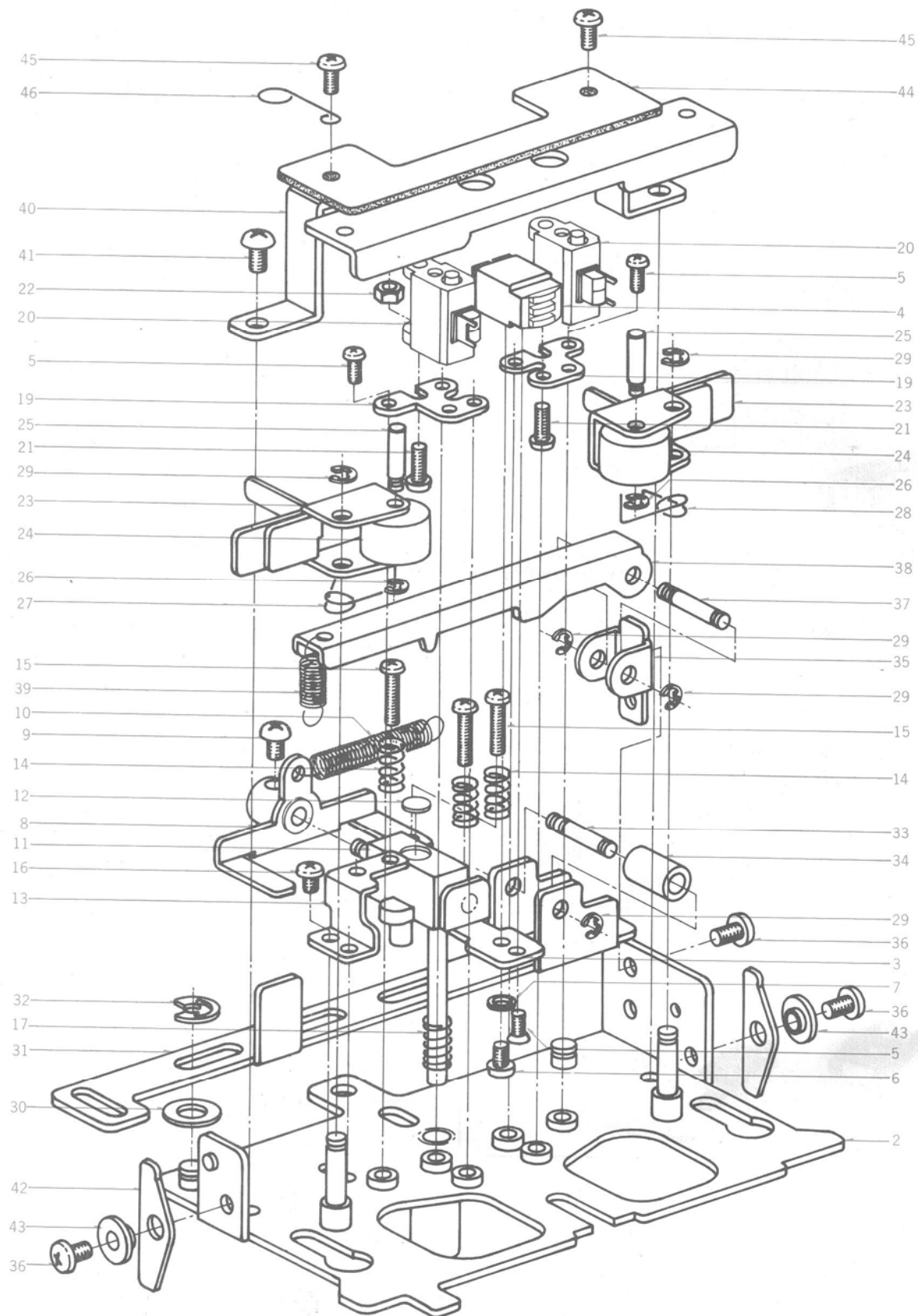
FIG. 1 ILLUSTRATION OF HEAD BLOCK
