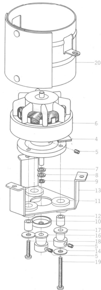
FIG. 2 ILLUSTRATION OF MOTOR BLOCK
