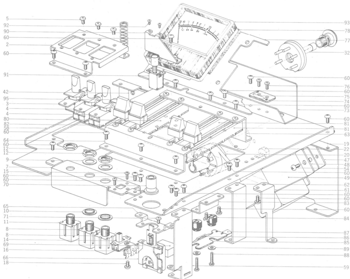
FIG. 12 ILLUSTRATION OF AMP. ASSEMBLY BLOCK
