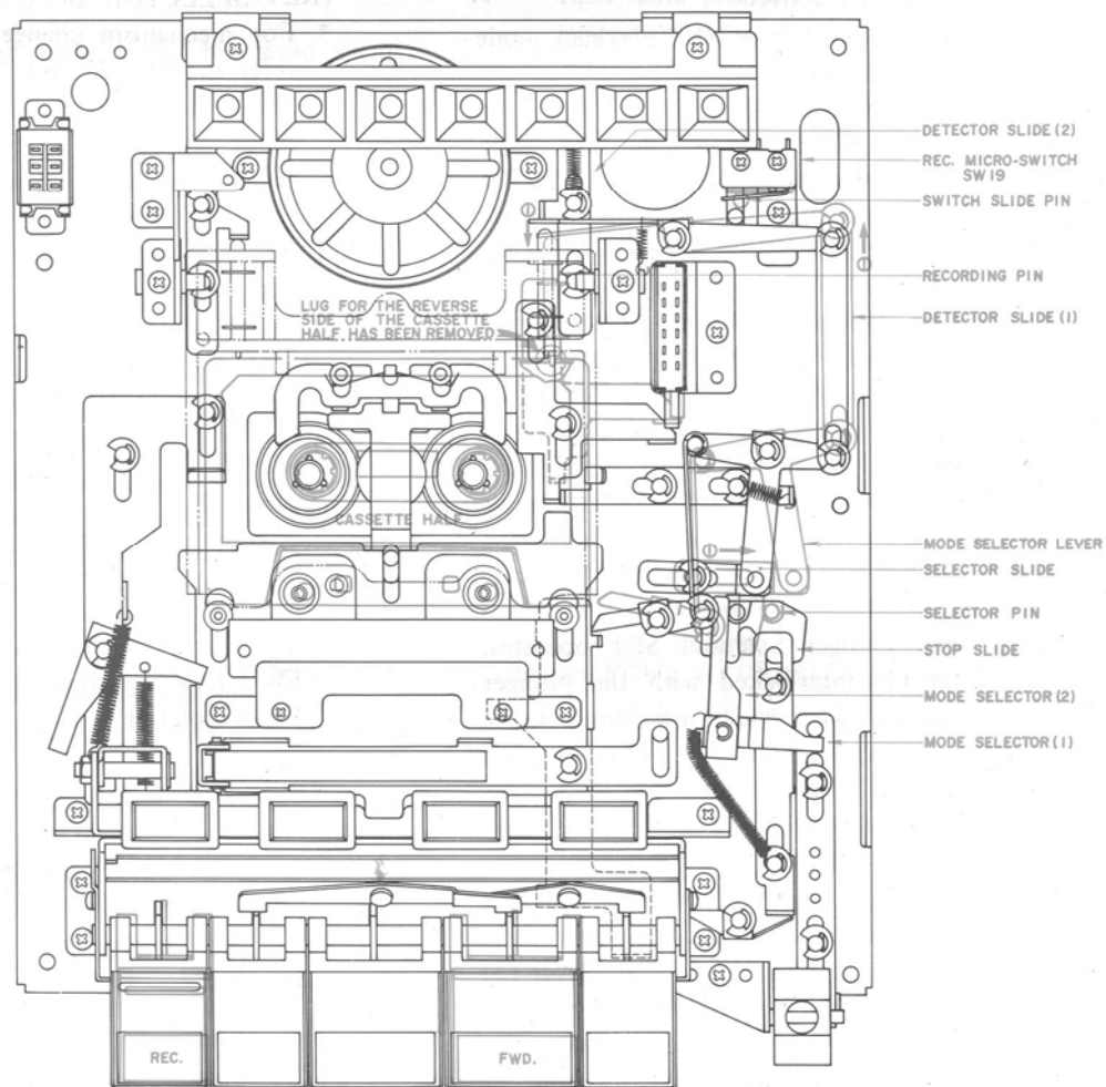
Fig. 36 Key Release From FWD REC Mode
