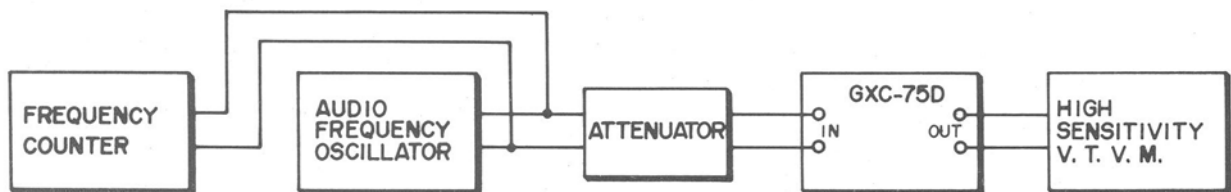
Fig. 21 Various Measuring Instrument Connections
