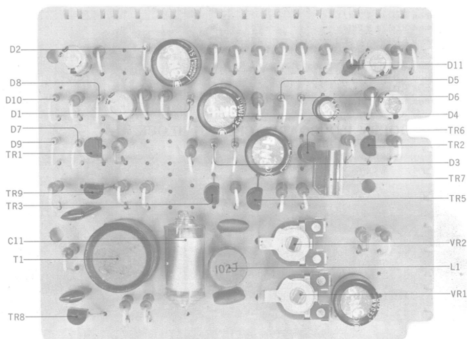
FIG. 10 PHOTO OF SYS. CON./OSC. P.C. BOARD (CP-2002) BLOCK
