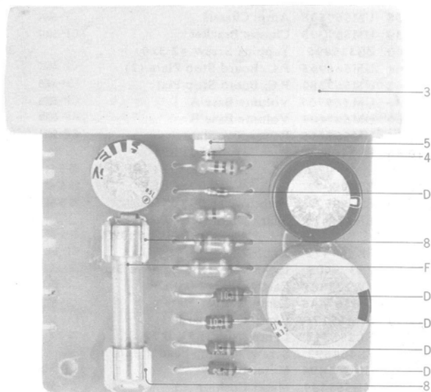
FIG. 11 PHOTO OF POWER SUPPLY P.C. BOARD (CP-5001) BLOCK
