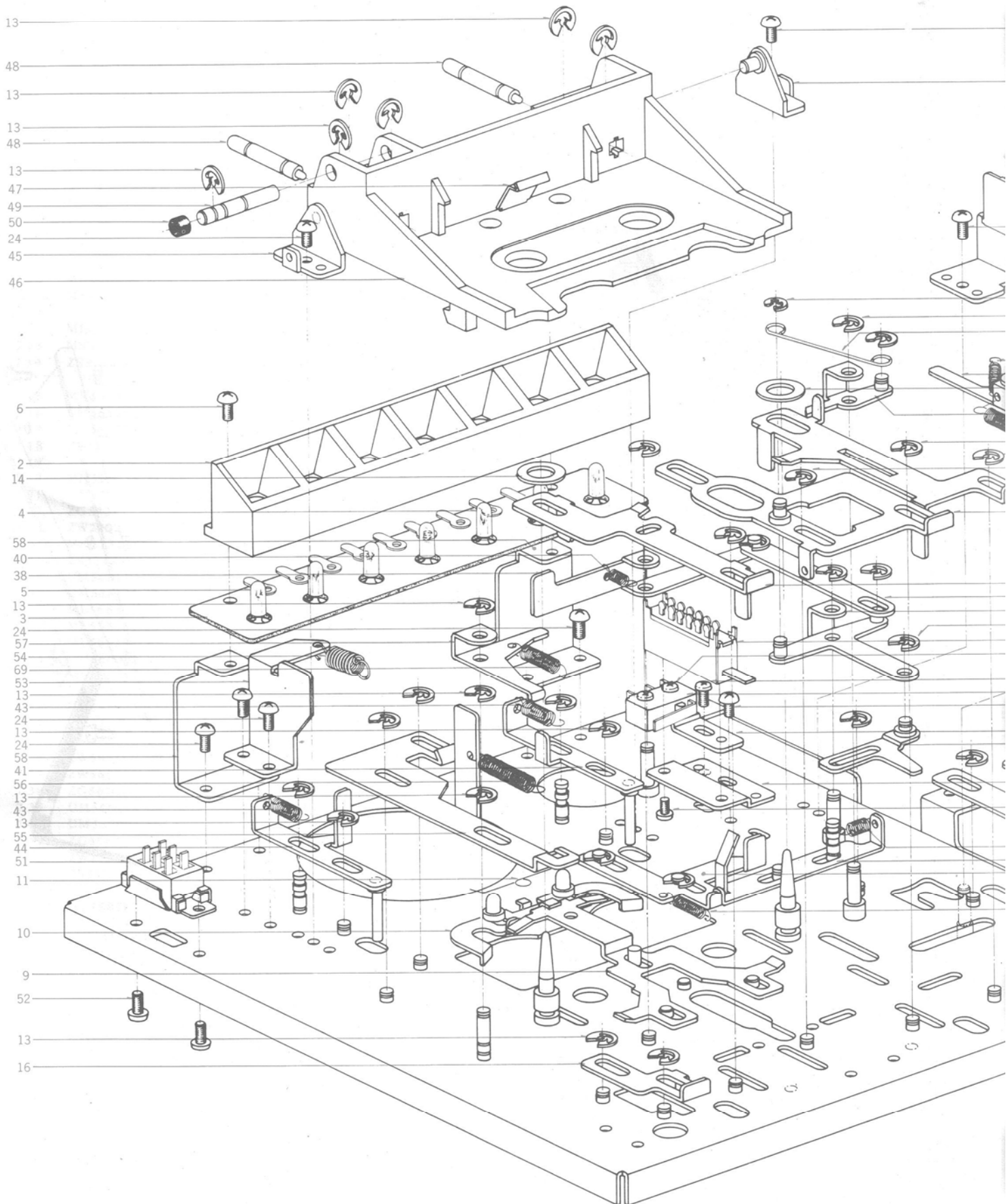
FIG. 6 ILLUSTRATION OF MECH. FRAME BLOCK (1)
