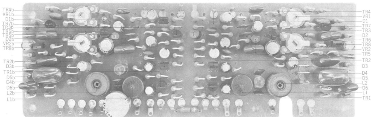
FIG. 9 PHOTO OF DOLBY P.C. BOARD (CP-5003) BLOCK
