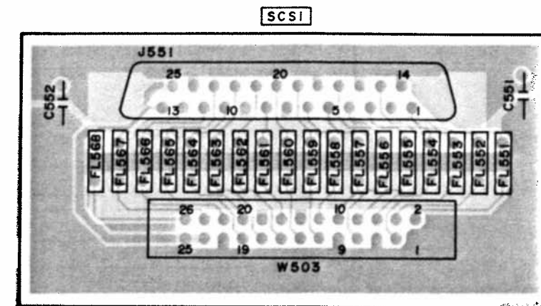
SCSI JACK PCB L40I2A506E
