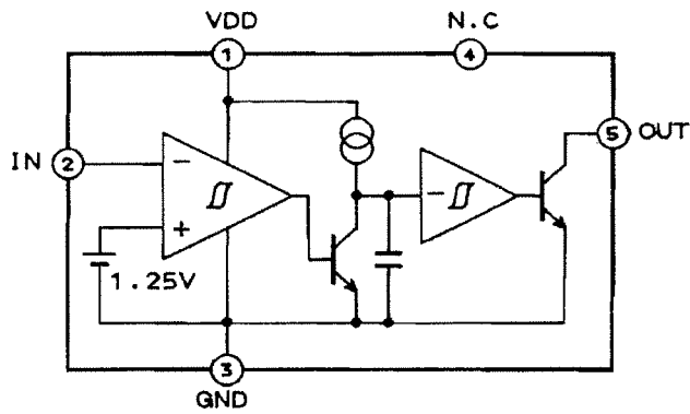
M51955BL (Reset pulse generator)
