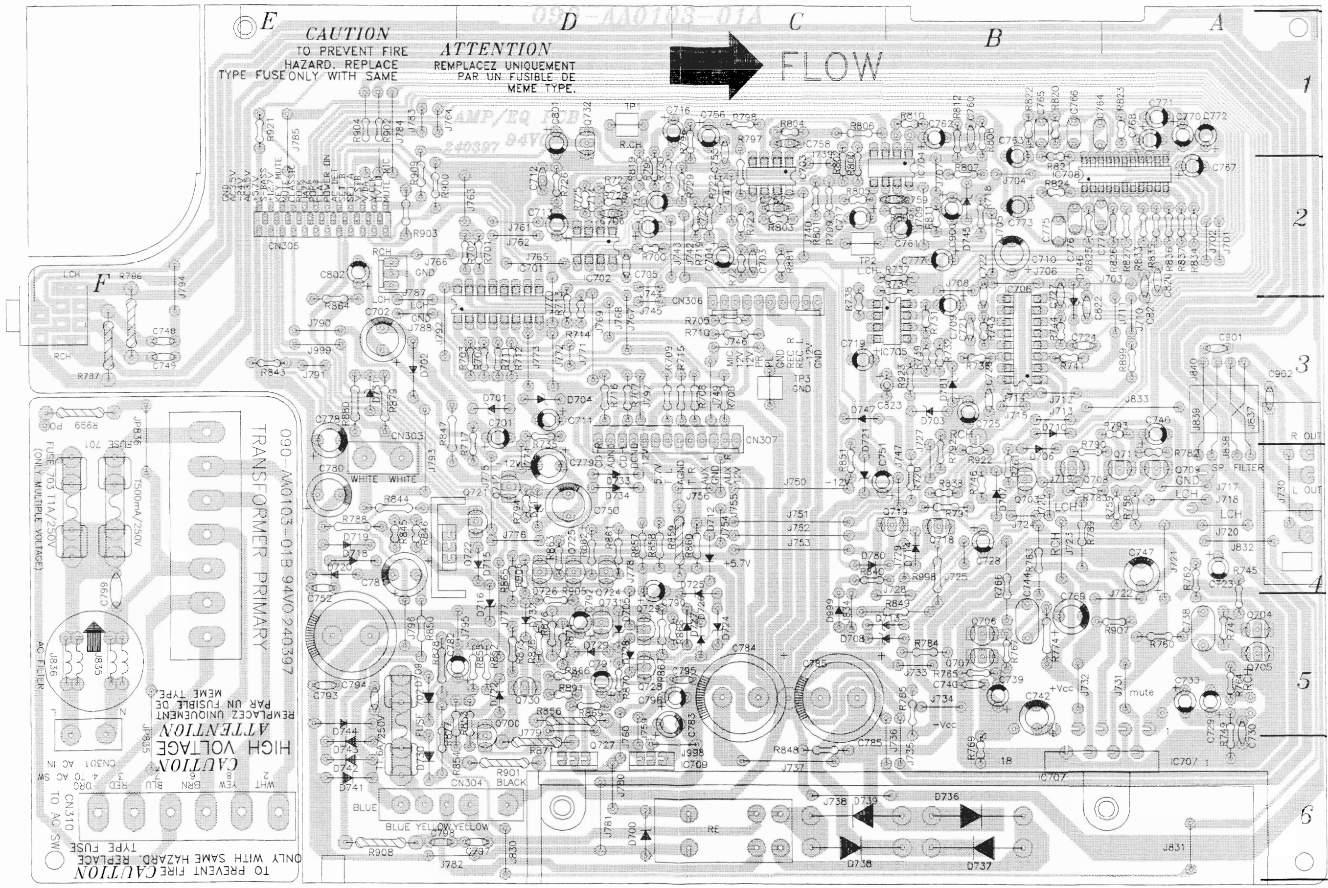
TOP VIEW
