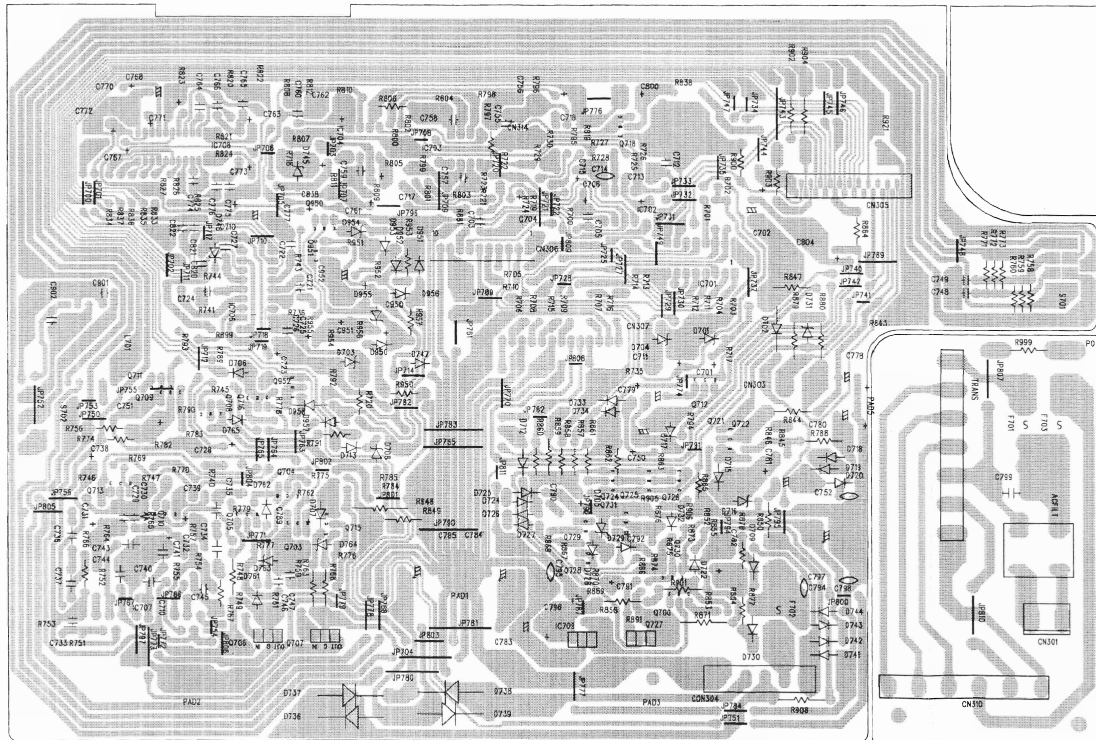
BOTTOM VIEW
