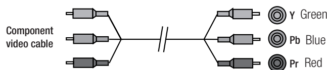
Figure 11 – Component Video
