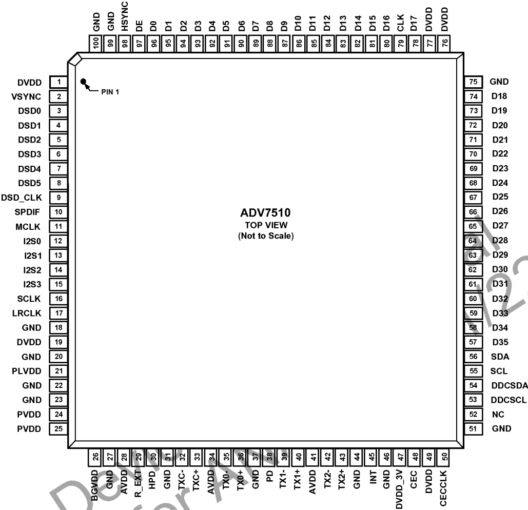
Figure 2. ADV7510 Pinout
