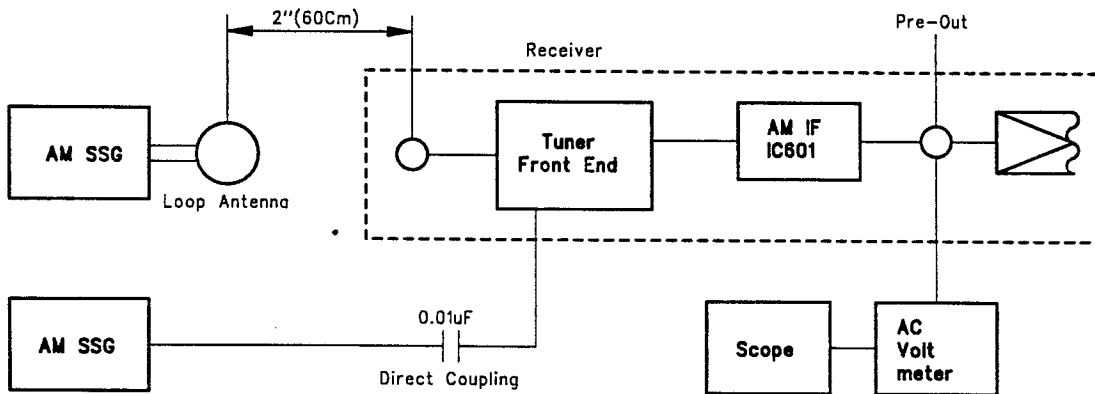
AM Alignment Connection
