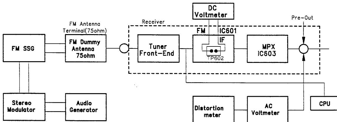
FM RF/IF and MPX Alignment Connection
