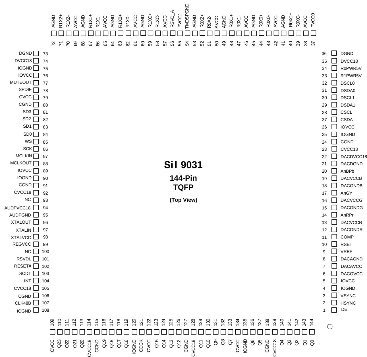
Figure 1. Pin Diagram
