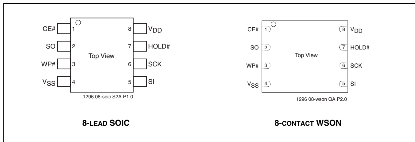
FIGURE 1: PIN ASSIGNMENTS
