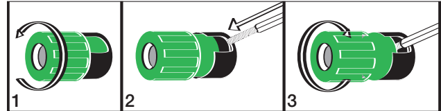
Figure 2 – Binding-Post Speaker Terminals With Bare Wires
