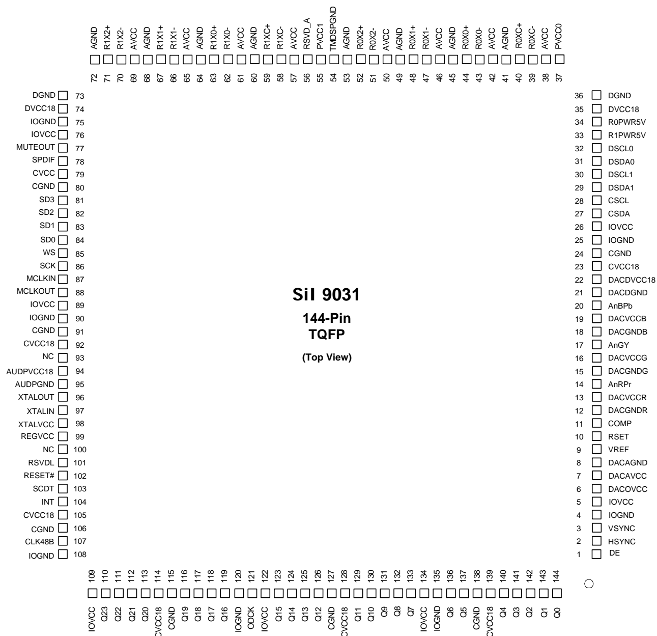
Figure 1. Pin Diagram
