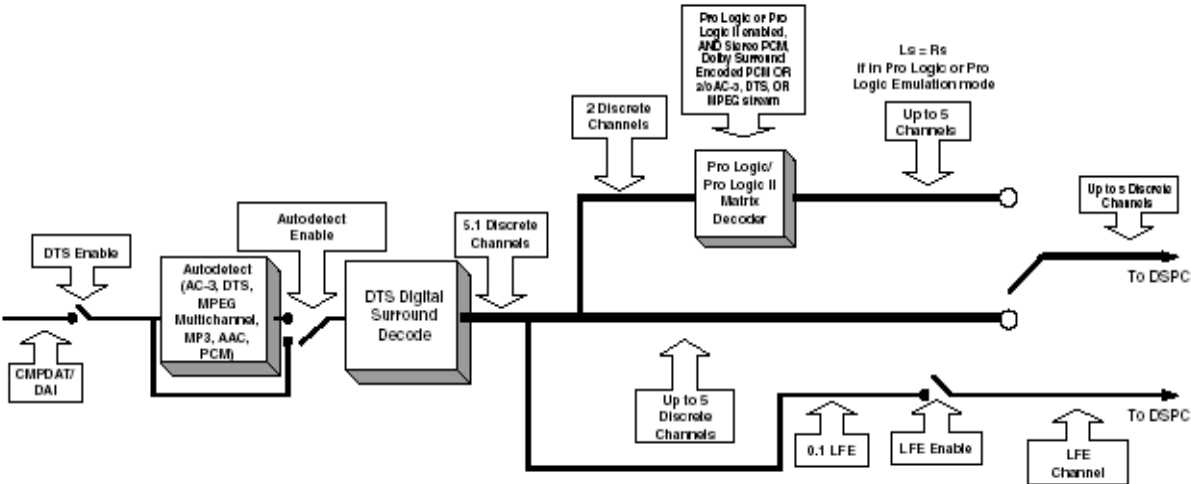
FIG 1-6 . DTS Block Diagram
