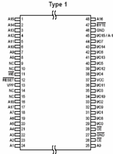
AT49BV/LV8192A(T) TSOP Top View
