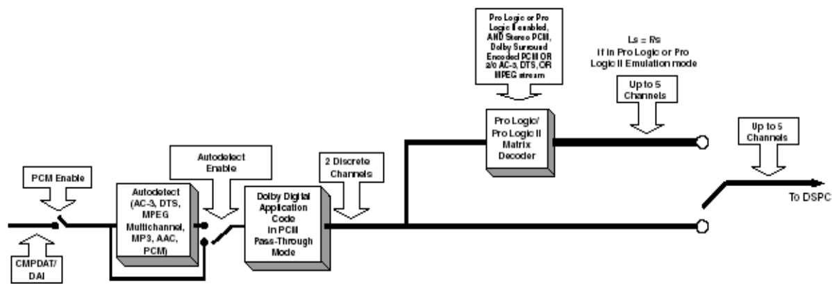
FIG 1-3 Dolby Digital Block Diagram, Configured for PCM Pass-Through
