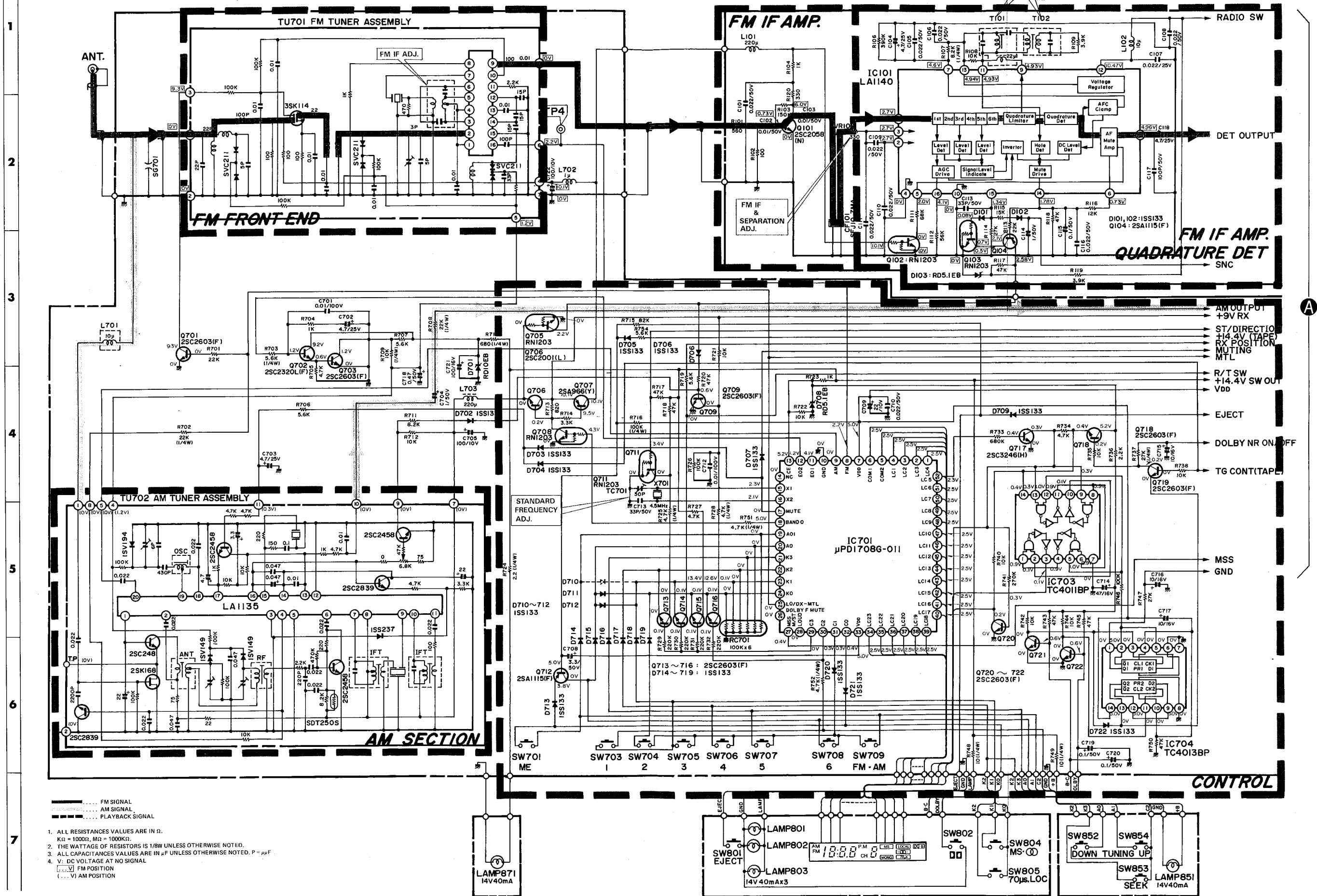
SCHEMATIC DIAGRAM (1)
