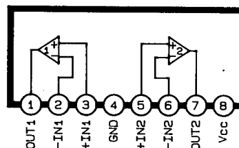
IC301 IC302 IC303 IC304 BA15218N (OP AMP)
