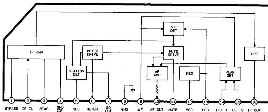
IC601 TA8129Z (FM IF AMP, PEAK DET)
