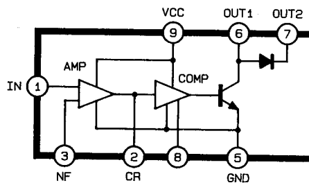
IC203 LA2000 (MUSIC SERCH)
