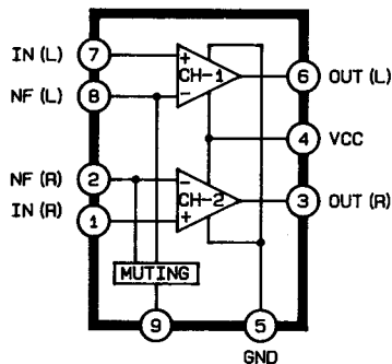
IC204 TA7325P (PLAYBACK AMP)
