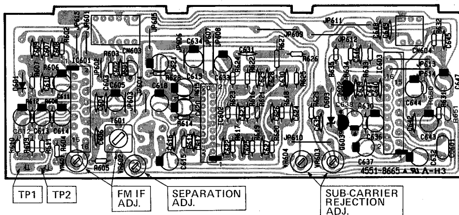
PCB-4
