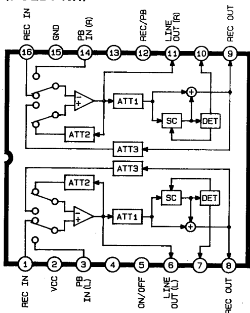
IC202 CXA1102F (DOLBY NR)
