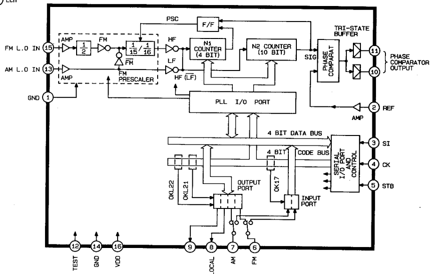
IC103 TC9172AP (PLL, PRE SCALER)
