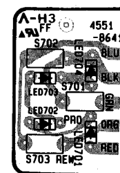
PCB-9 PRO/FF/REW SWITCH P.C. BOARD
