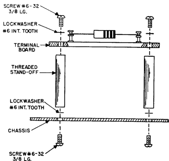
TERMINAL BOARD ASSEMBLY FIGURE L
