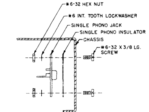
DOUBLE PHONO JACK ASSEMBLY SIMILAR EXCEPT FOR ADDITION OF GROUND LUG SHOWN ON PICTORIAL 4 PHONO JACK ASSEMBLY
