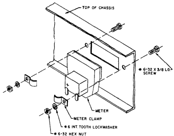
METER ASSEMBLY FIGURE H
