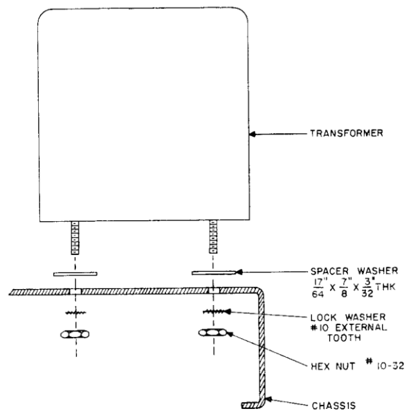
TRANSFORMER ASSEMBLY FIGURE K
