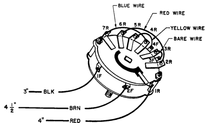
PRELIMINARY SWITCH WIRING FIGURE J
