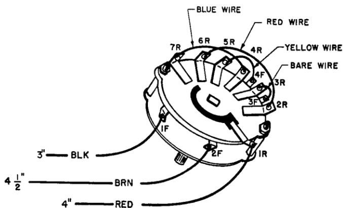
PRELIMINARY SWITCH WIRING FIGURE J
