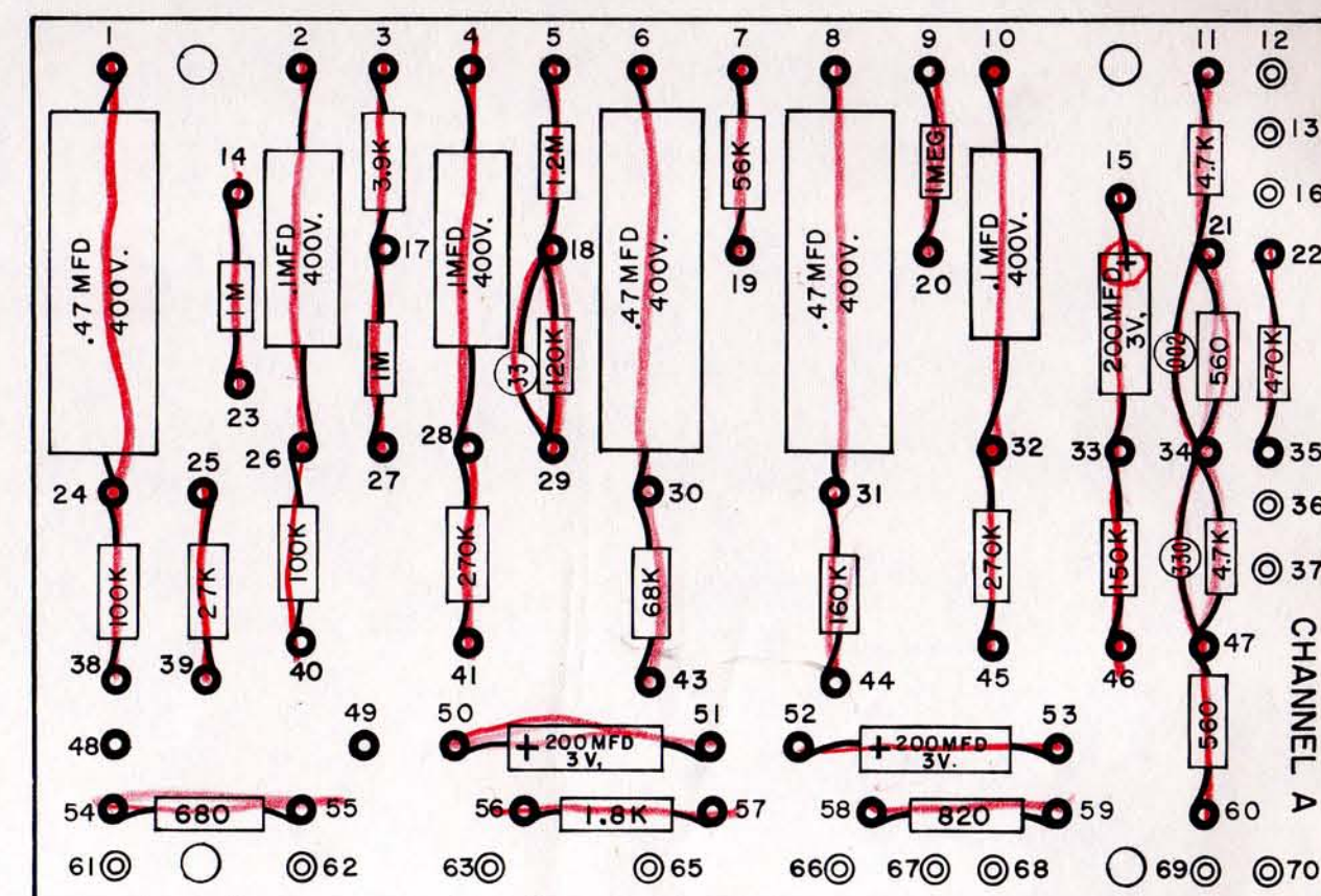
FIG. C TOP OF BOARD (COMPONENTS MTG.)
