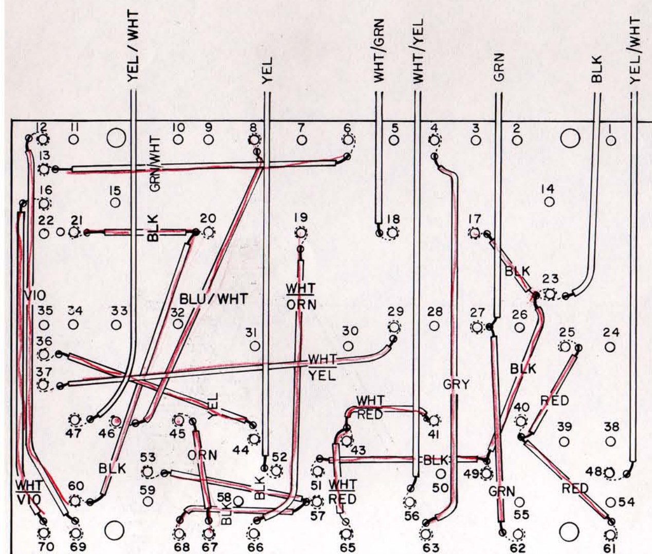
FIG. A BOTTOM OF BOARD (WIRING)
