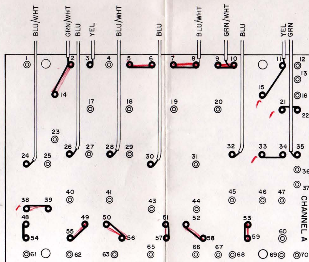
FIG. B TOP OF BOARD (WIRING) CHANNEL A
