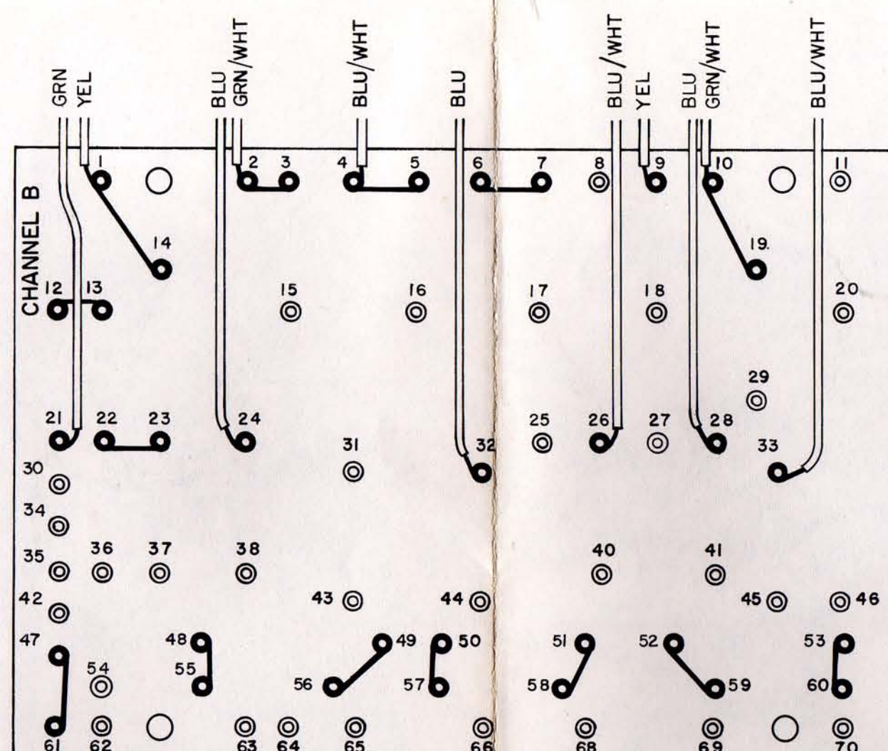
FIG. E TOP OF BOARD (WIRING) CHANNEL B
