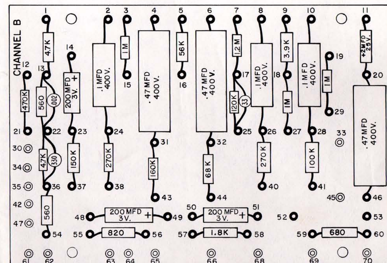
FIG. F TOP OF BOARD (COMPONENTS MTG)
