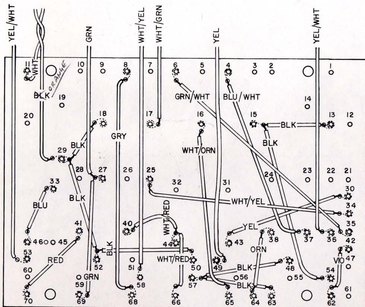
FIG. D BOTTOM OF BOARD (WIRING)
